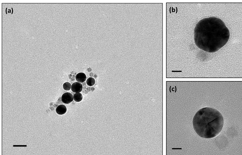
Figure S1. (a) TEM image of Au-Fe 3 O 4 nanocomposites. The sizes of Fe 3 O 4 and Au nanoparticles are around 10 nm and 30 nm, respectively; (b,c) TEM images of a single Au-Fe 3 O 4 nanocomposite; The scale bars are 50 nm, 10 nm and 10 nm in (a-c), respectively.
