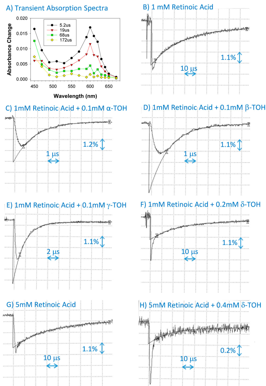
Figure 3. Transient absorption spectra at indicated times after pulse radiolysis of N_2O -saturated benzene with 1 mM of solubilized retinoic acid (A), and representative kinetics monitored at 600 nm (B–H) of the formation and decay of retinoic acid cation radicals after pulse radiolysis in the absence and presence of \alpha -tocopherol ( \alpha -TOH), \beta -tocopherol ( \beta -TOH), \gamma -tocopherol ( \gamma -TOH), and \delta -tocopherol ( \delta -TOH).
