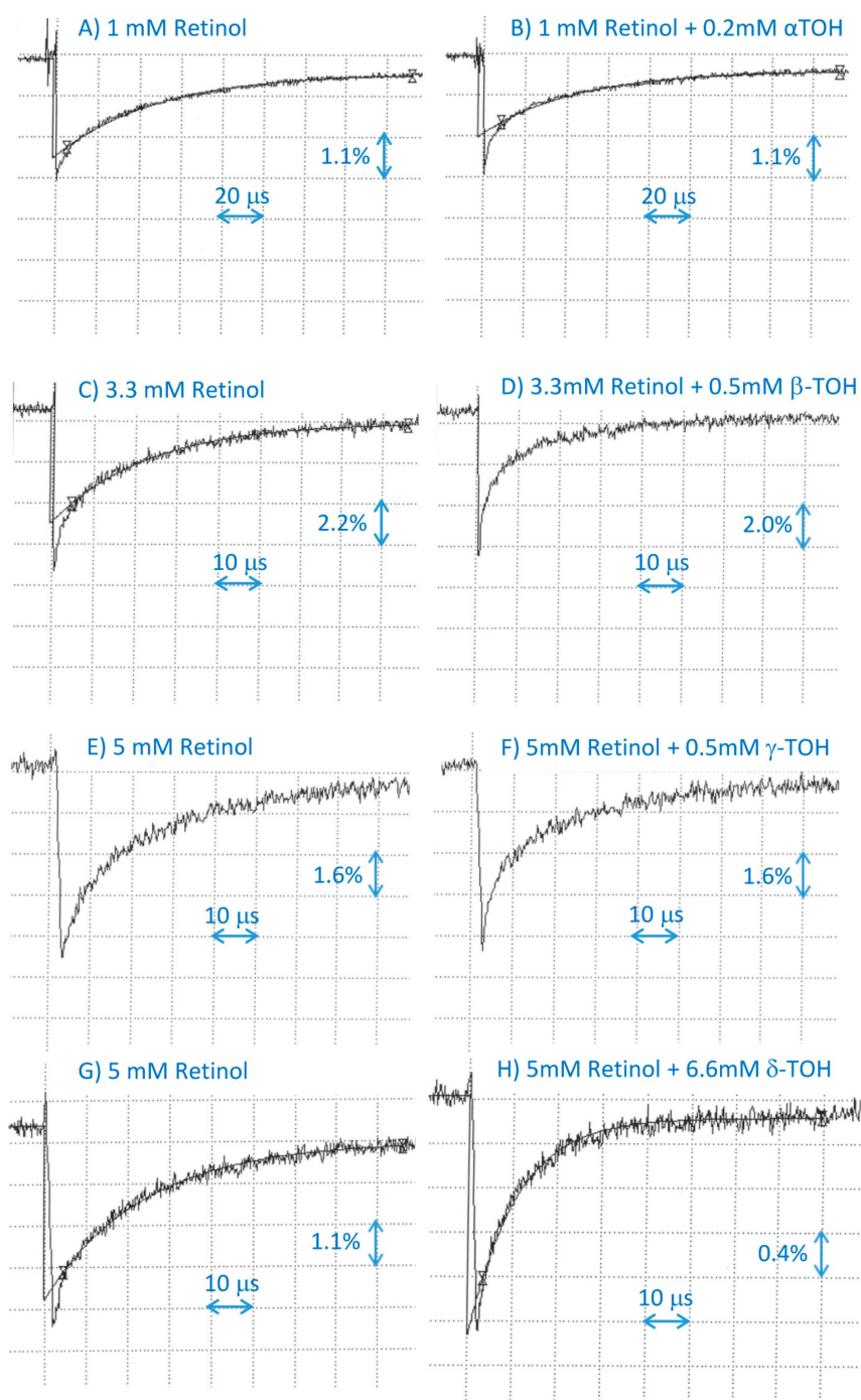
Figure 5. Representative kinetics of the formation and decay of retinol cation radicals monitored at 610 nm after pulse radiolysis of N_2O -saturated benzene with solubilized retinol at indicated concentrations in the absence (A,C,E,G) and presence of \alpha -tocopherol ( \alpha -TOH, B), \beta -tocopherol ( \beta -TOH, D), \gamma -tocopherol ( \gamma -TOH, F), and \delta -tocopherol ( \delta -TOH, H).
