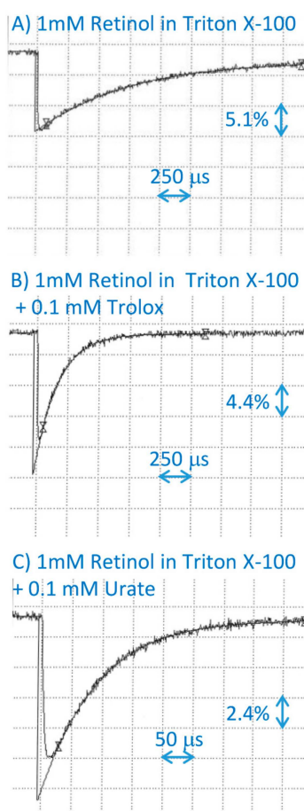
Figure 6. Representative kinetics of the formation and decay of retinol cation radicals monitored at 590 nm after pulse radiolysis of aqueous solution saturated with \text{N}_2\text{O} and containing 10 mM of phosphate, pH 7, 0.1 M of KBr, and 1 mM of retinol incorporated in 2% Triton X-100 micelles, in the absence (A) and presence of 0.1 mM of Trolox (B) or uric acid (C).
