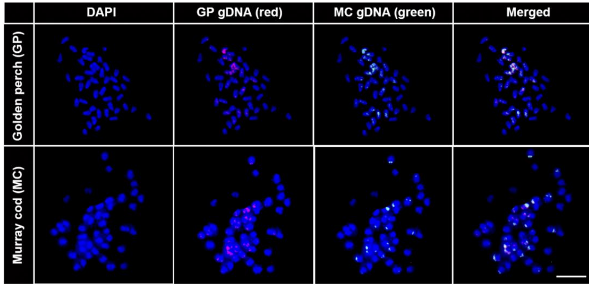
Figure S1. Cross-species CGH of golden perch and Murray cod. Red signals represent hybridisation of golden perch genomic DNA and green signals represents hybridisation pattern of Murray cod in metaphase chromosome of both species. Scale bar 5 \mu m
