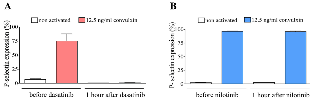
Figure S1. Dasatinib completely abolished the effect of convulxin on alphagranule excretion. Samples were from dasatinib (n=3) or nilotinib (n=3) treated CML patients before and at 1 h after witnessed drug administration. Platelets of patients were stimulated with convulxin in PRP. Alphagranule excretion was investigated by monoclonal antibody against P-selectin. Columns show the mean and SEM.
