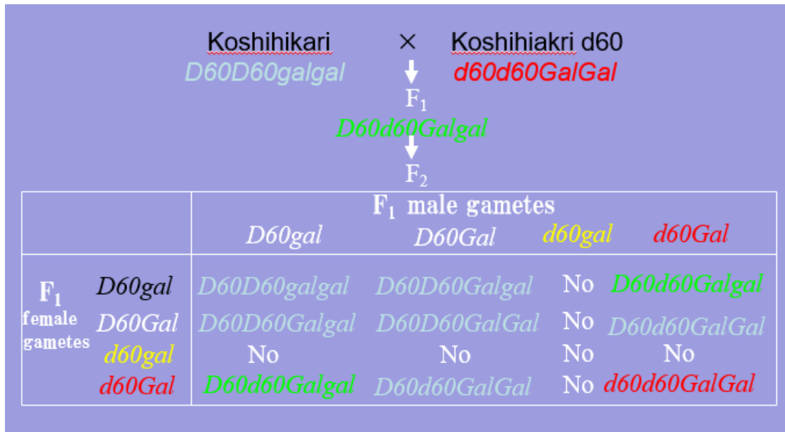
Figure S1. Complementary gamete lethal between semidwarfing gene d60 and gamete lethal gene gal .
