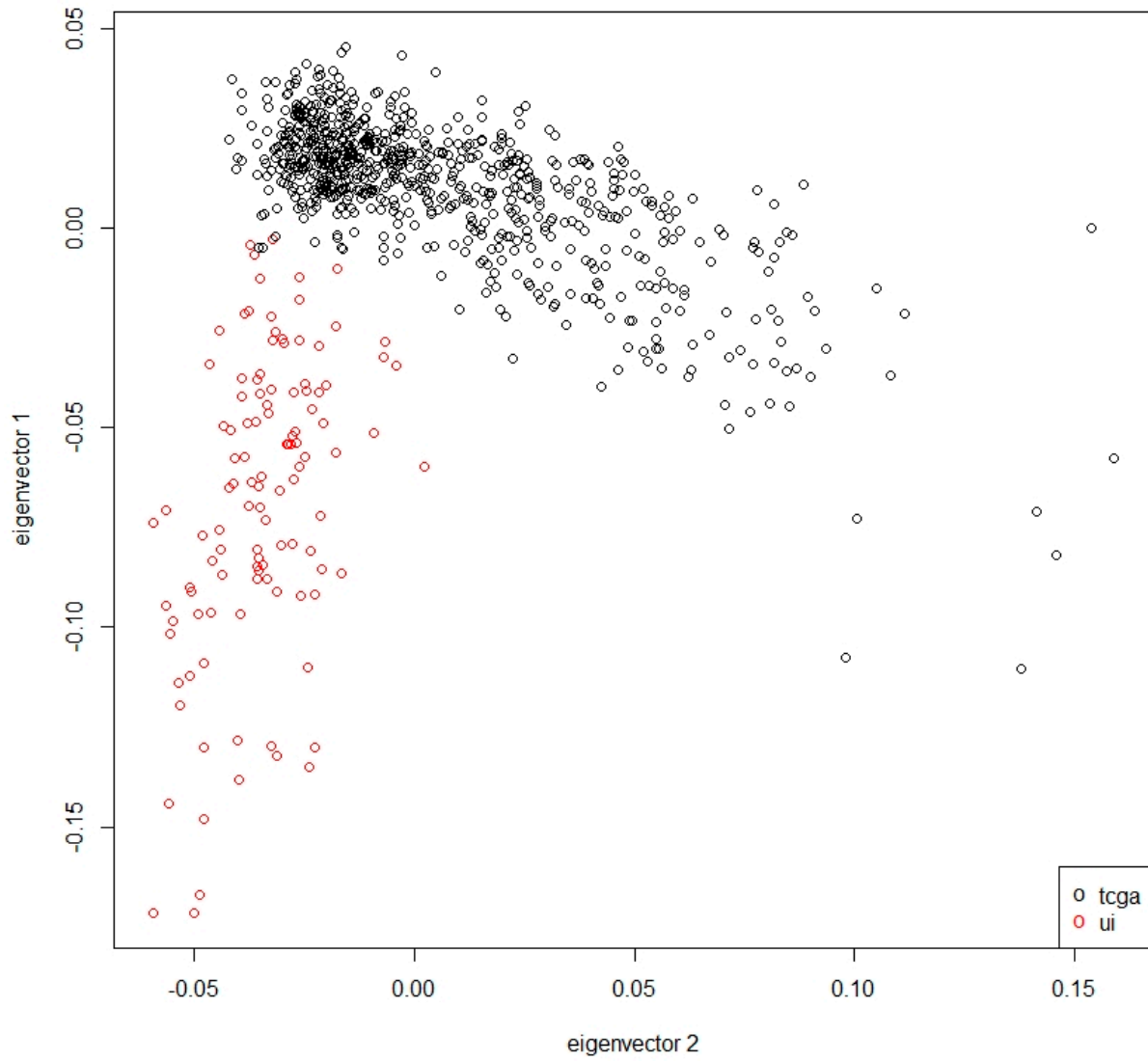
Figure SB1: Representation of the first two eigenvectors of the PCA analysis between UIHC and TCGA cohorts. The first two eigenvectors hold the largest percentage of variance between both cohorts and the total variance accounted for is over two-thirds of the total. ui: UIHC cohort; tcga: TCGA cohort.
