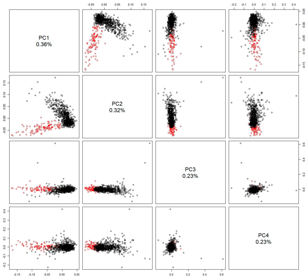
Figure SB2: Representation of the principal component pairs for the first four principal components.
