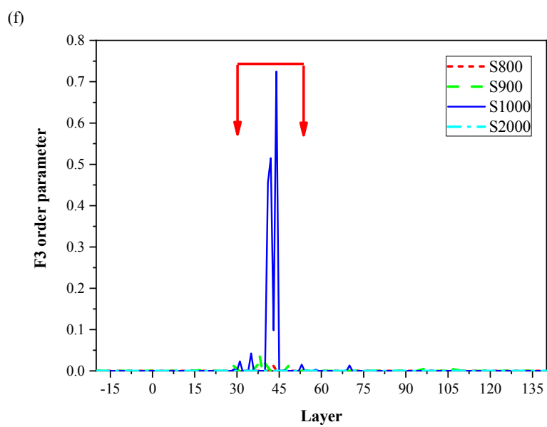
Fig. S1 F3 order parameter for 2 \times 2 \times 10 unit cells of different sI methane hydrate systems during stretching. (a) deletion percentage of 0.91%; (b) deletion percentage of 1.99%; (c) deletion percentage of 2.69%; (d) deletion percentage of 3.07%; (e) deletion percentage of 5.92%; (f) deletion percentage of 9.02%.
