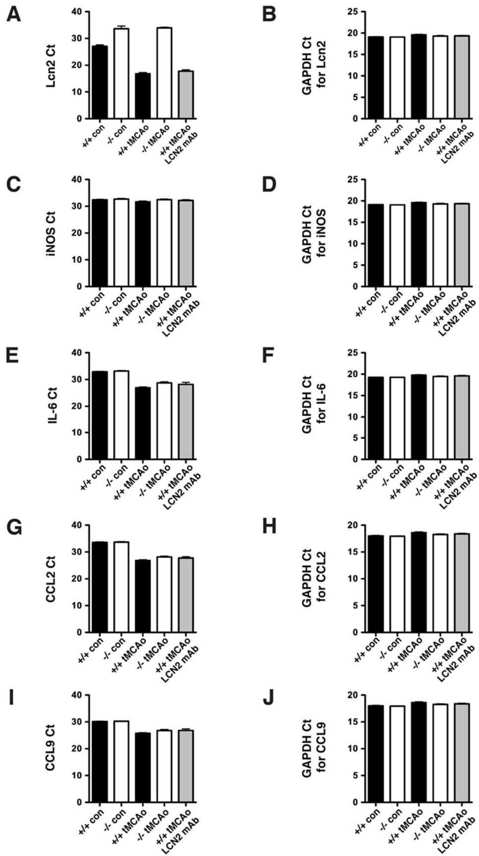
Figure S1. Ct values of qPCR results for LCN2 (A), iNOS (C), IL-6 (E), CCL2 (G), CCL9 (I) and their associated GAPDH's (B,D,F,H,J).
