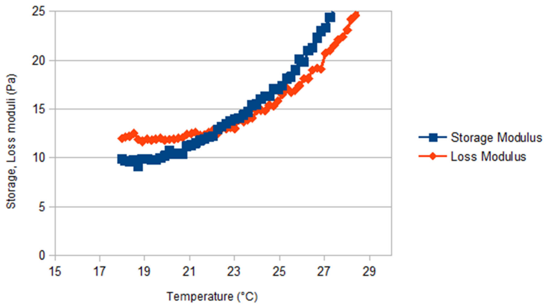
Figure S1. Representative storage and loss moduli values as a function of temperature for 20% placebo hydrogels. The figure shows that at the temperature of 22.4 °C the value of storage
