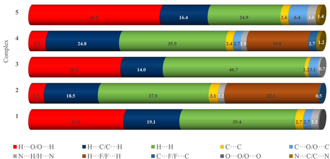
Figure 6. The percentage of non-covalent interactions for the analysed complexes extracted from 2D fingerprint plots.
