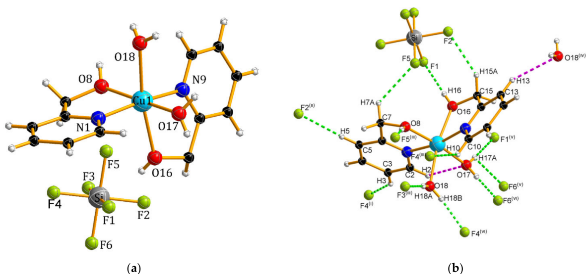
Figure 2. (a) Molecular structure of [\text{Cu}(2\text{-(HOCH}_2\text{)py})_2(\text{H}_2\text{O})_2]\text{SiF}_6 ( 2 ) and (b) the hydrogen bonding formed by the water molecules and hexafluorosilicate ions in complex 2 .
