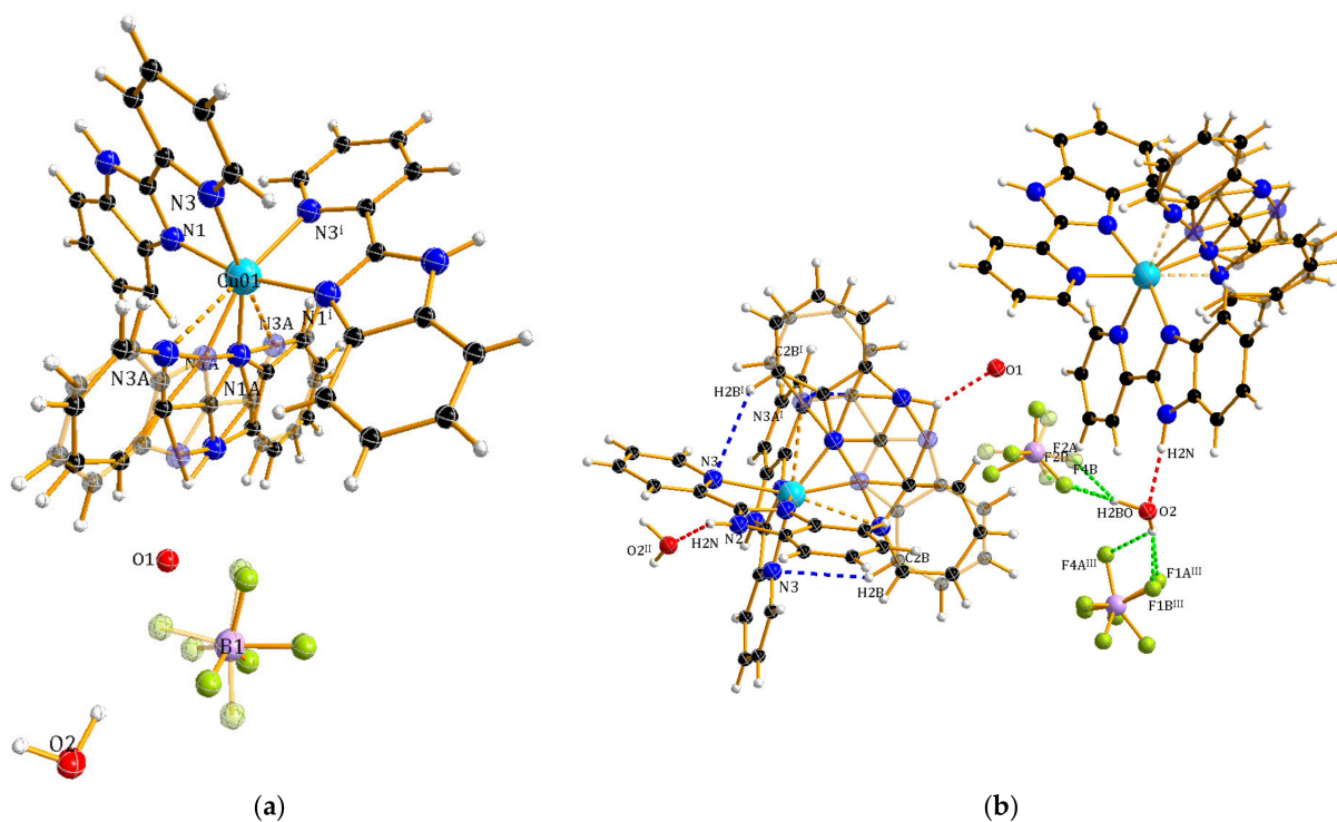
Figure 4. (a) Molecular structure of [\text{Cu}(\text{pyBIm})_3](\text{BF}_4)_2 \cdot 1.5\text{H}_2\text{O} (4) and (b) selected intra- and intermolecular H-bonding interactions.
