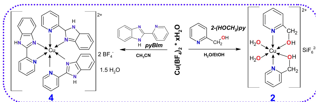
Scheme 2. Schematic representation of copper(II) complexes synthesis from copper(II) tetrafluoroborate hydrate.
