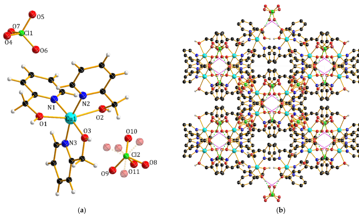
Figure 1. Perspective view of (a) the molecular structure and (b) the crystal packing with marked O-H...O/Cl bonds of [\text{Cu}(2\text{-(HOCH}_2\text{)py})_3](\text{ClO}_4)_2 (1).
