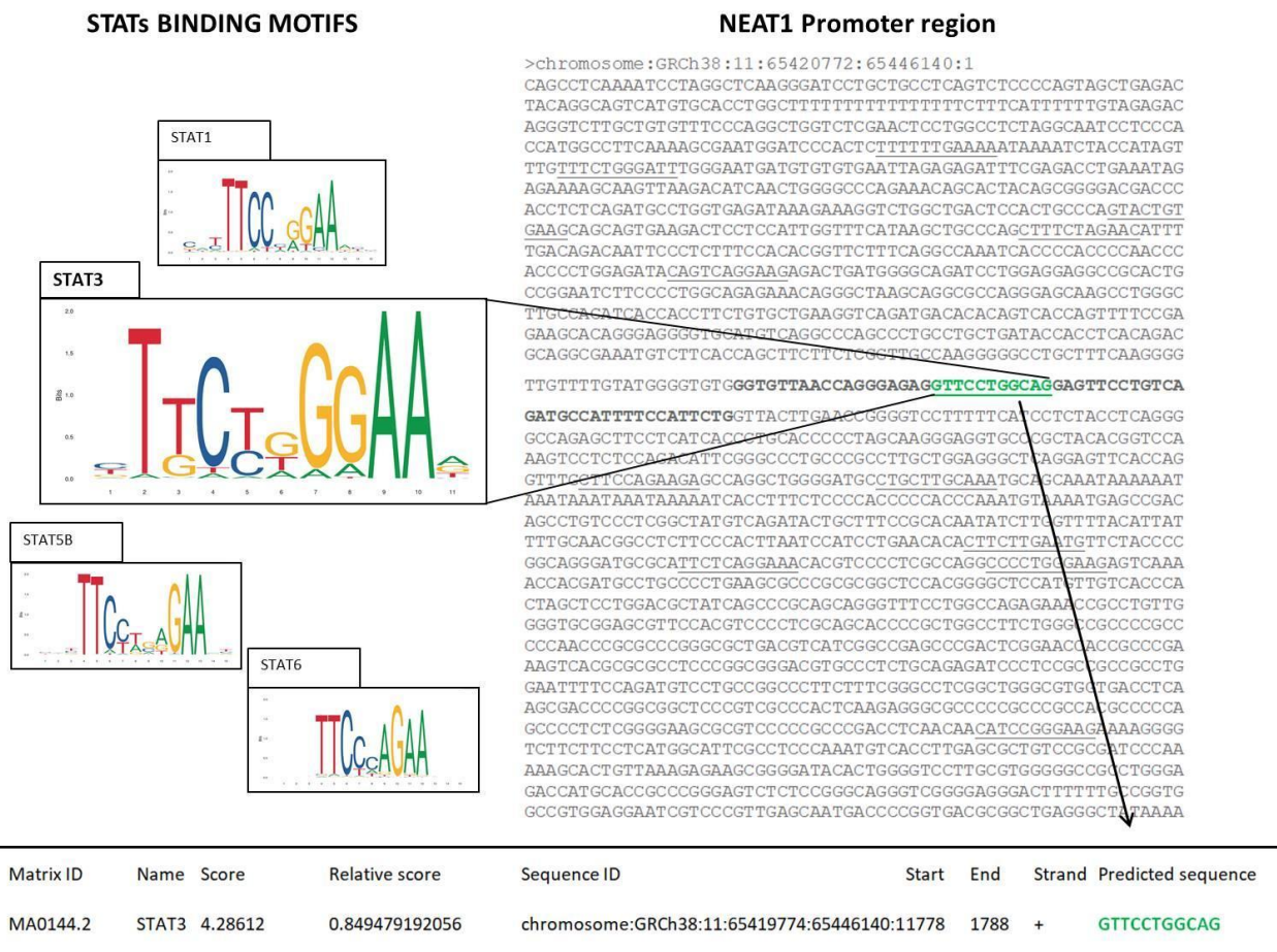
Figure S2. Identification of STAT family binding motif in NEAT1 promoter by Jaspar program. Common STATs binding motifs are reported on the left. On the right: raw FASTA sequence of NEAT1 promoter with STAT3 motifs underlined. The promoter region chosen to design gel shift biotinylated probes is in bold, the chosen STAT3 binding motif is highlighted in green. Predicted sequence location and relative score are reported as Jaspar prediction output.
