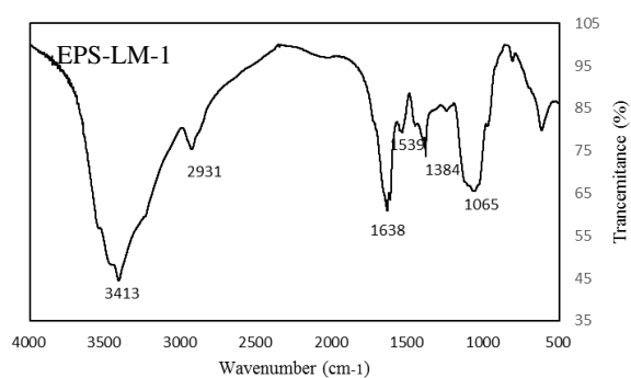
Figure S2. FT-IR spectrum of EPS-LM-1.
