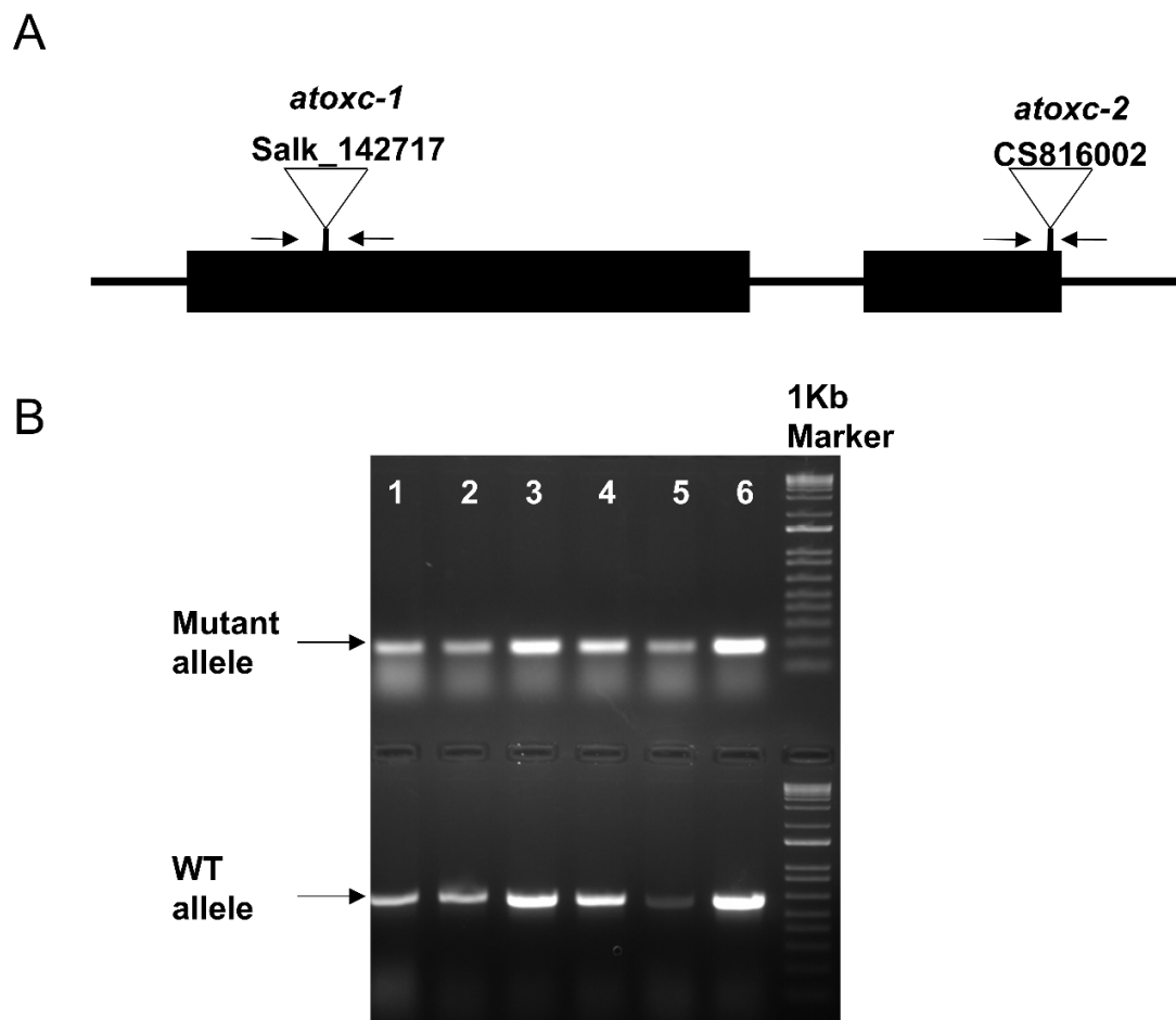
Figure S1. Analysis of two T-DNA insertional lines of AtOXC gene. (A) Diagram indicates the first allele (Salk_142717) and the second allele (SAIL_343_D06) of AtOXC T-DNA insertional lines. Arrows indicate the genotyping PCR primers. (B) PCR genotyping of Basta resistant individual plants of T3 SAIL_343_D06 line, showing all individual plants carry both T-DNA insertion and WT allele.
