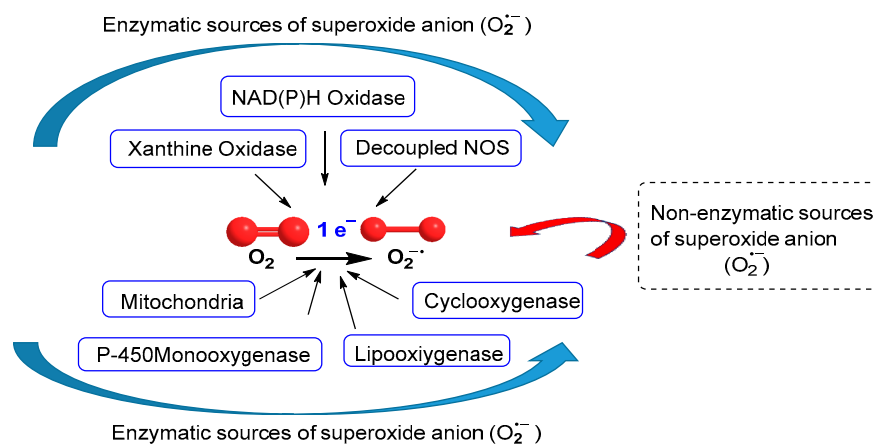
Figure 8. Enzymatic sources of superoxide anion and non-enzymatic production of superoxide [25].
