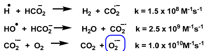
Figure 21. The CO_2^{\bullet-} formed reduces the O_2 to O_2^{\bullet-} .
