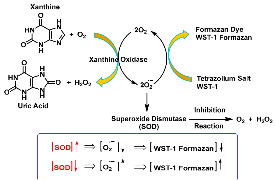
Figure 41. SOD inhibition assay mechanism.
