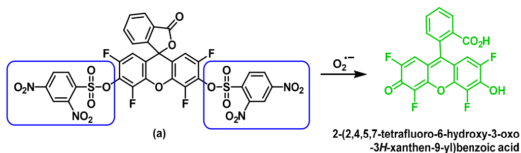
Figure 66. Mechanism of fluorescent response of probe (a) to O_2^{\bullet-} .
