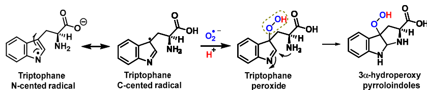
Figure 56. Trp • reacts with O 2 •- , the major products being hydroperoxides.
