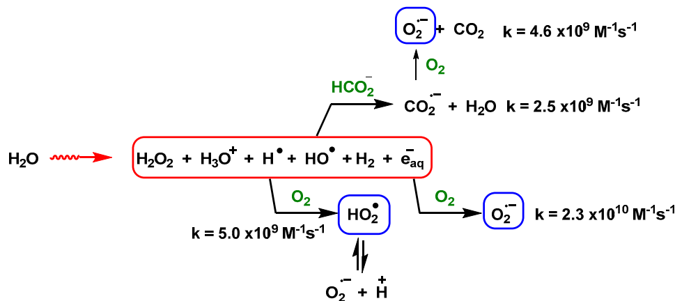
Figure 18. The radiolysis of water is performed under high-energy electrons and if the water contains molecular oxygen and sodium formate, the primary radicals become O_2^{\bullet-}/HO_2^{\bullet} .
