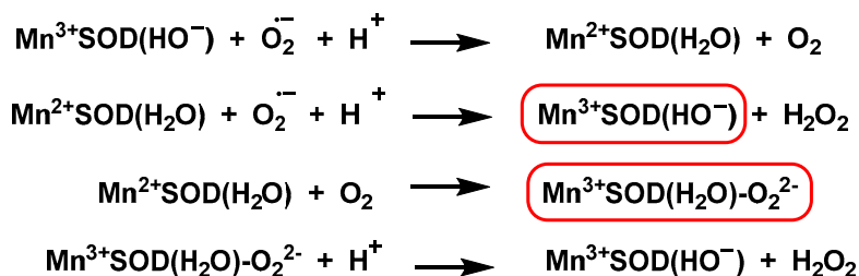
Figure 36. The mechanism includes the formation of both \text{Mn}^{3+}\text{SOD} and the complex ( \text{Mn}^{3+}\text{SOD}(\text{H}_2\text{O})\text{-O}_2^{2-} ).
