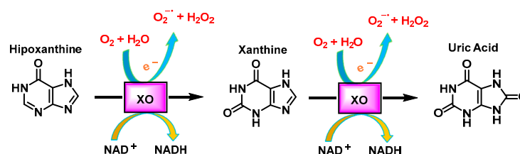
Figure 15. Reactions catalysed by xanthine oxidase.
