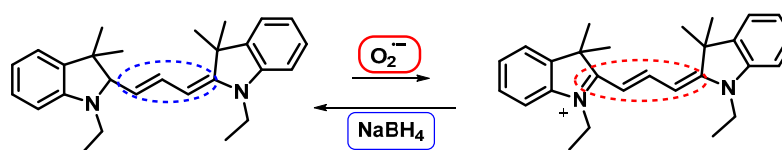
Figure 70. The oxidation–reduction reaction of hydrocyanines and cyanines.
