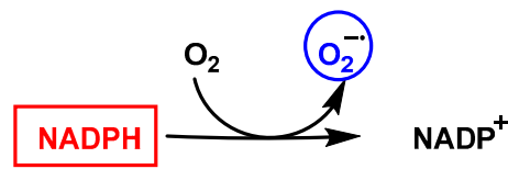
Figure 12. Reduction of O_2 to O_2^{\bullet-} by NADPH.
