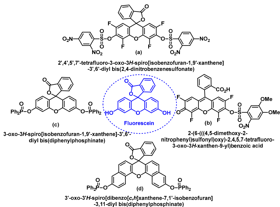
Figure 65. Four fluorescein-derived probes used for O_2^{\bullet-} detection.
