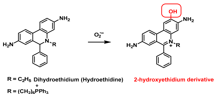
Figure 62. Fluorescent response mechanism of the dihydroethidium (hydroethidium) probe and derivatives to \text{O}_2^{\bullet-} .
