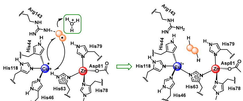
Figure 35. Second part of the reaction mediated by SOD1, transformation of the second \text{O}_2^{\bullet-} into hydrogen peroxide and regeneration of the catalytic centre.
