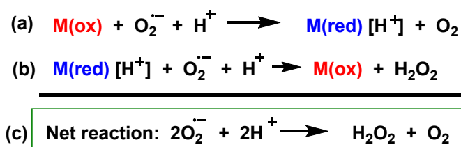
Figure 31. SOD-mediated reaction mechanism: (a) elimination of the first superoxide anion and reduction of copper; (b) second part of the reaction of transformation of the second peroxide anion into hydrogen peroxide and regeneration of the catalytic centre; (c) net reaction. Where M(ox) is the oxidized state of the metal in the catalytic centre ( \text{Cu}^{2+} , \text{Zn}^{2+} or \text{Mn}^{3+} ), and M(red) denotes the reduced state of the same metal ( \text{Cu}^+ , \text{Zn}^{2+} or \text{Mn}^{2+} ).
