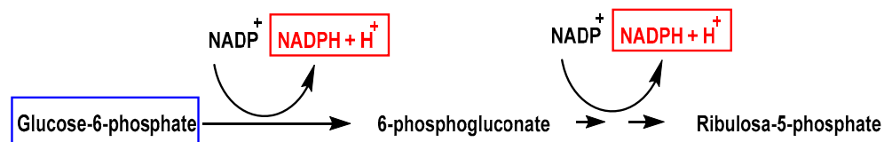
Figure 11. Formation of NADPH molecule in the transformation of glucose-6-phosphate into ribulose 5-phosphate.
