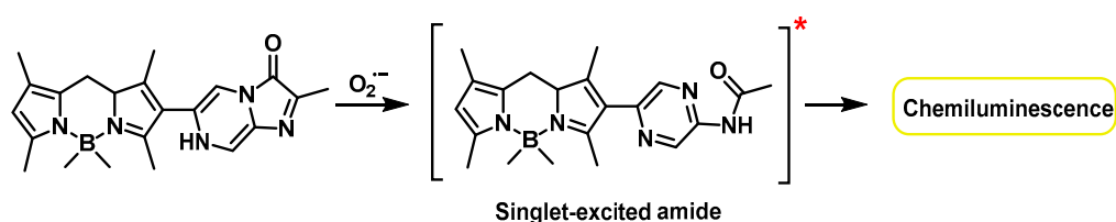
Figure 68. Mechanism of chemiluminescence response of probe BODIPY.
