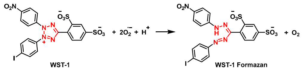
Figure 42. Structure of WST-1 (4-(3-(4-iodophenyl)-2-(4-nitrophenyl)-2H-tetrazol-3-ium-5-yl) benzene-1,3-disulfonate).
