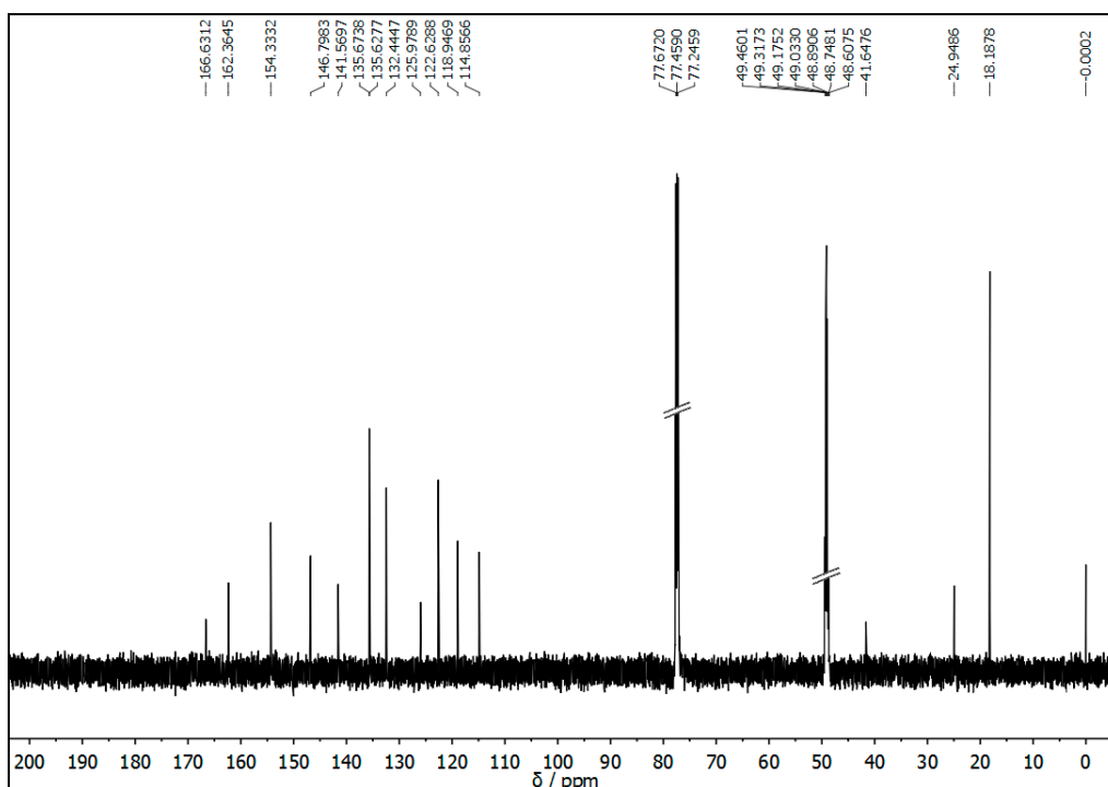
Figure S2. ^{13}\text{C} -NMR spectrum of 4 in \text{CDCl}_3/\text{MeOD-}d_4 .
