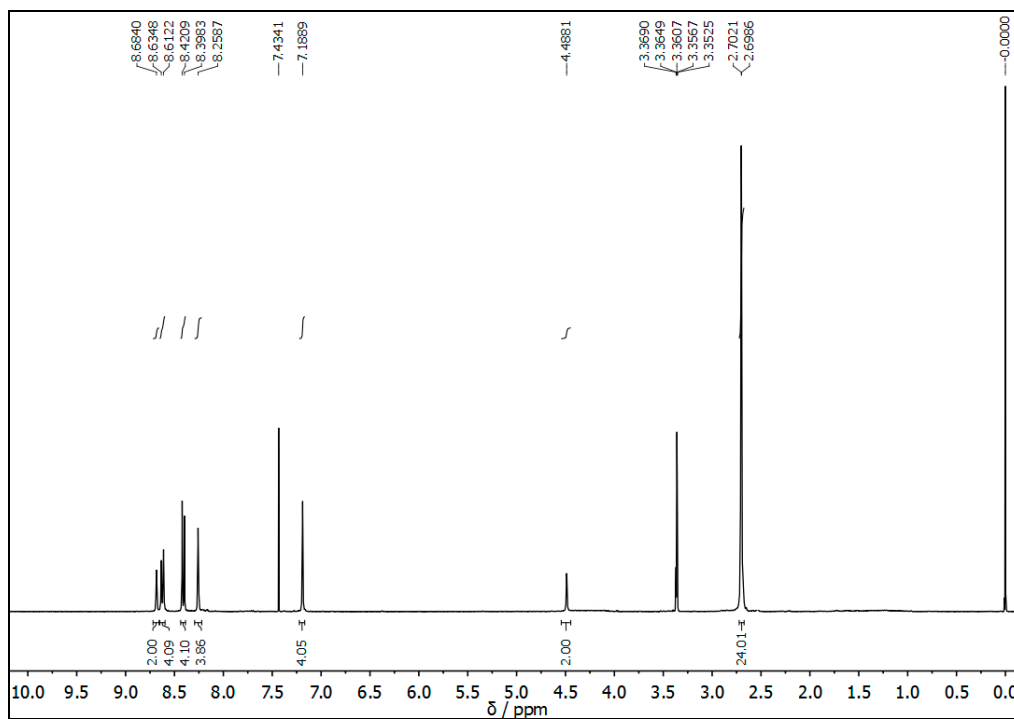
Figure S1. ^1\text{H} -NMR spectrum of 4 in \text{CDCl}_3/\text{MeOD-}d_4 (400 MHz).
