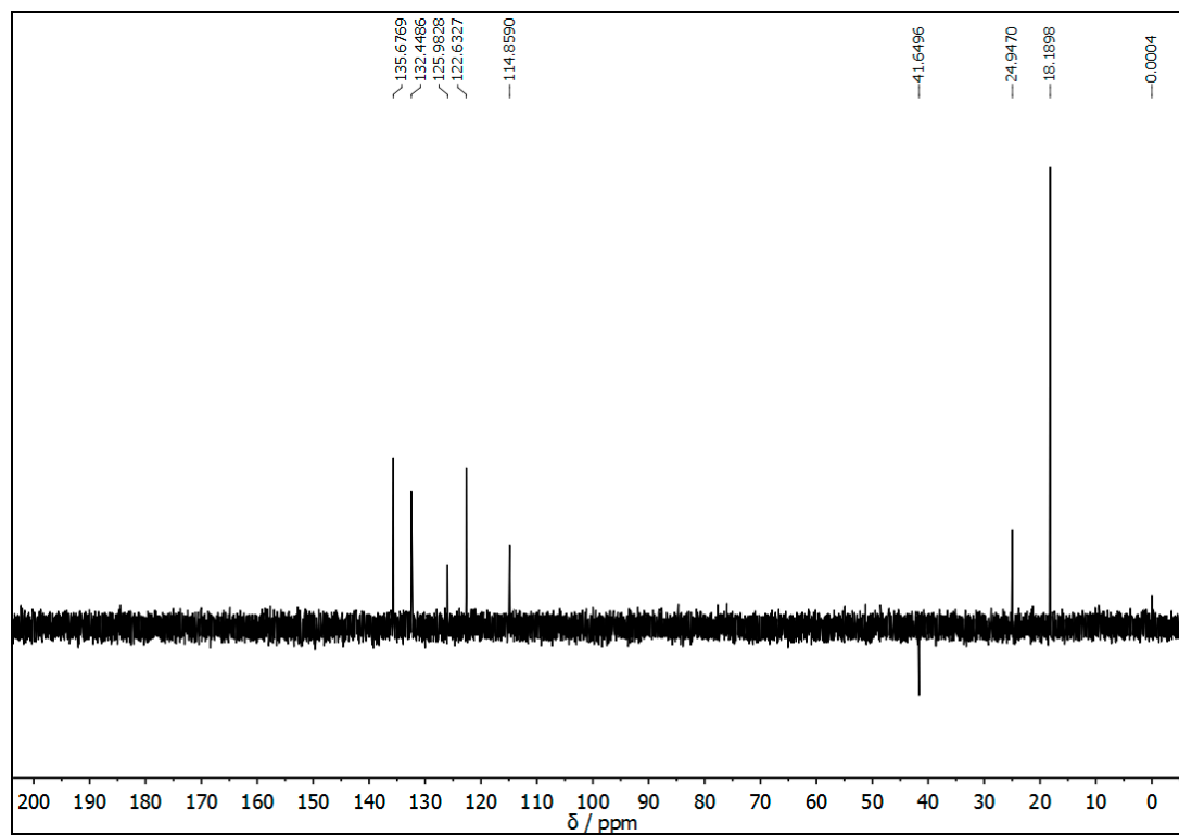
Figure S3. DEPT spectrum of 4.
