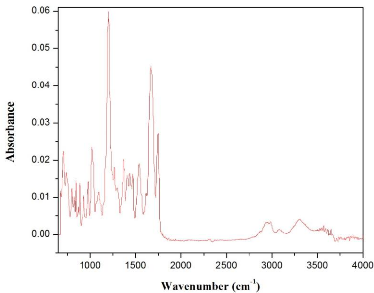
Figure S2. FTIR spectrum of ethyl([acryloyl(furan-2-ylmethyl)amino]acetyl)amino)acetate.
