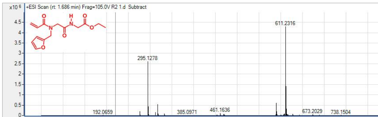
Figure S1. LCMS spectra of ethyl([acryloyl(furan-2-ylmethyl)amino]acetyl)amino)acetate.
