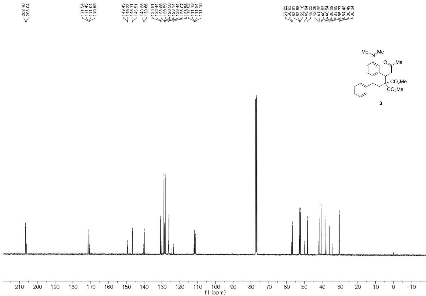
Figure S2. 13 C-NMR spectrum of 3 (CDCl 3 , 100 MHz)
