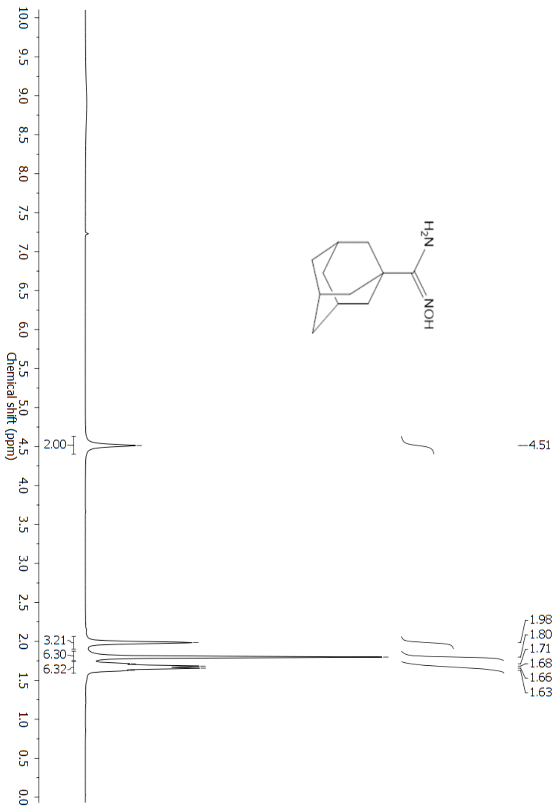
Figure S1. ^1\text{H-NMR} spectrum of 3 .
