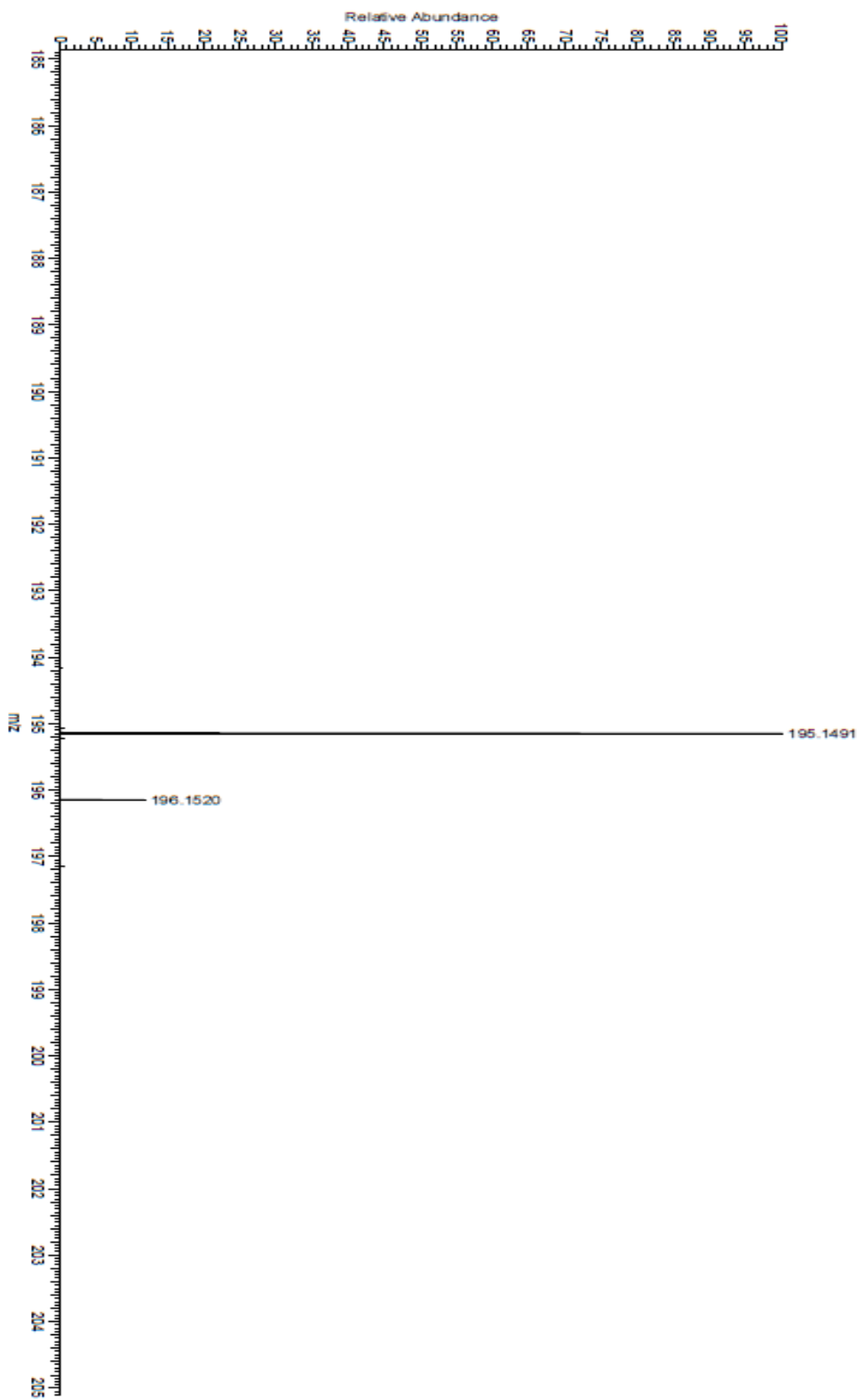
Figure S4. High-resolution mass spectrum of 3.
