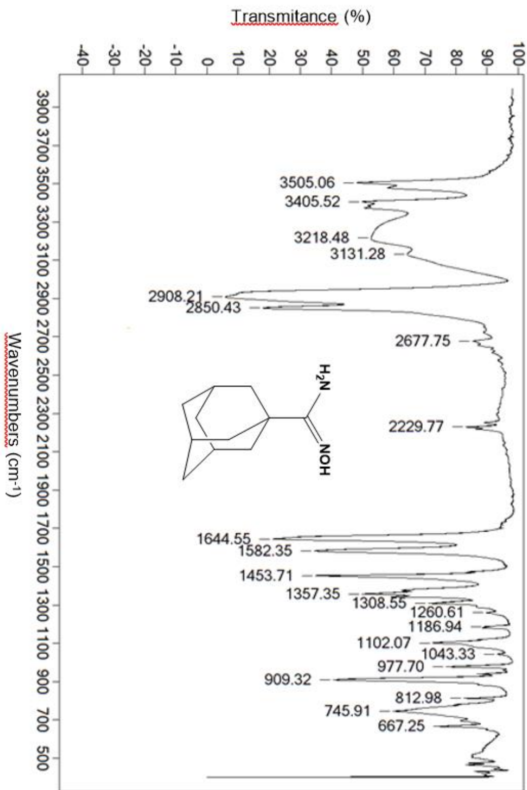
Figure S3. IR spectrum of 3.
