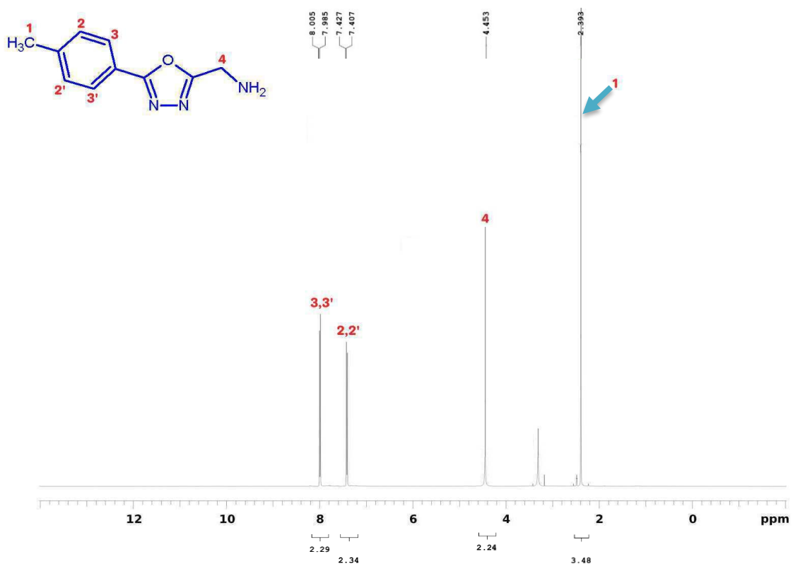
Figure S1. 1 H-NMR spectra of 1-[5-(4-tolyl)-1,3,4-oxadiazol-2-yl]methanamine (Compound 3)
