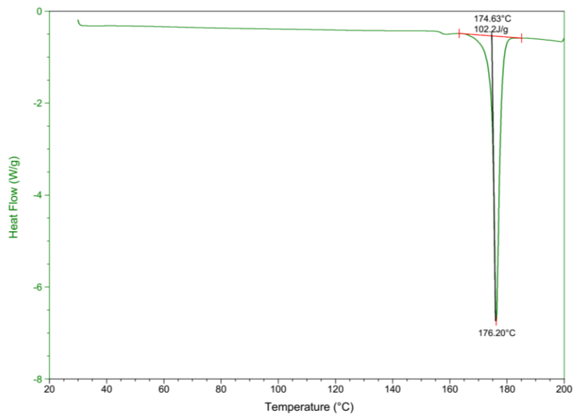
Figure S5. DSC spectrum of 1-[5-(4-tolyl)-1,3,4-oxadiazol-2-yl]methanamine (Compound 3)
