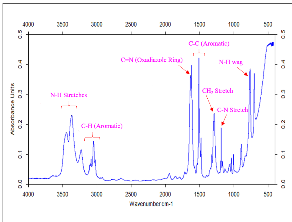
Figure S4. FTIR spectrum of 1-[5-(4-tolyl)-1,3,4-oxadiazol-2-yl]methanamine (Compound 3)
