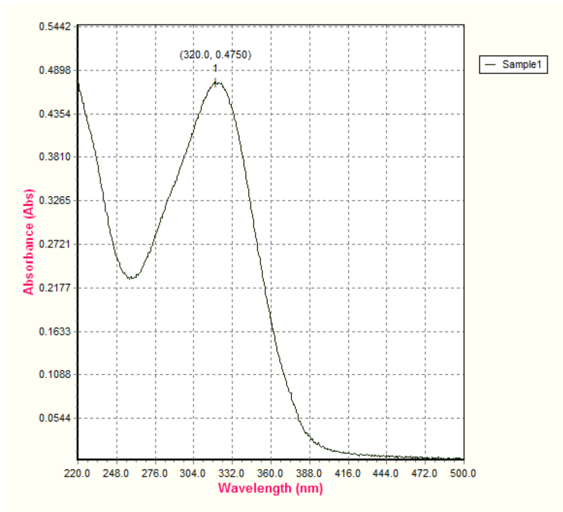
Figure S1: UV spectrum of (E) -1-(2',4'-dimethyl)-(5-acetylthiazole)-(2'',4''-difluorophenyl)-prop-2-en-1-one in HCl.
