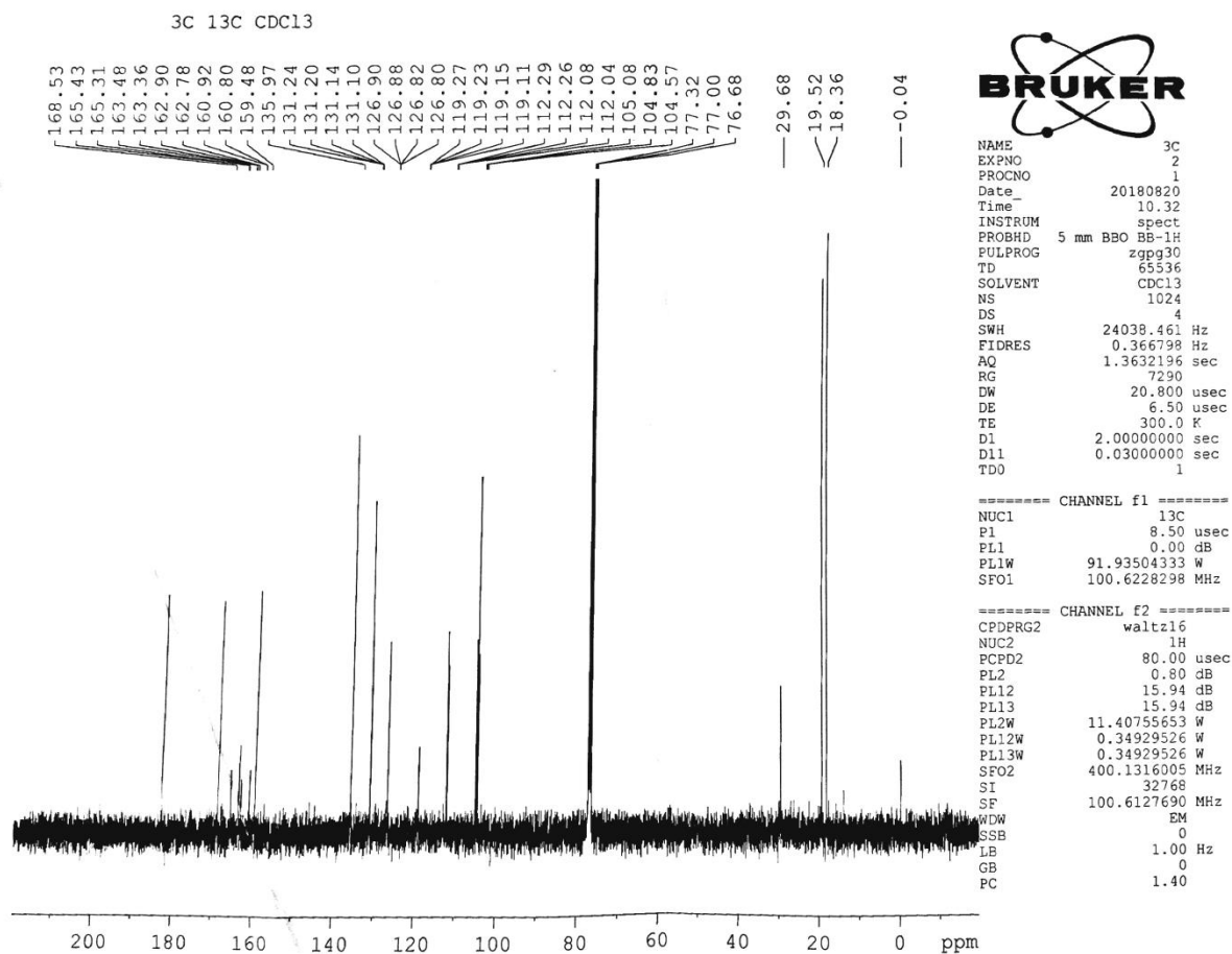
Figure S4: ^{13}\text{C} -NMR spectrum of ( E )-1-(2',4'-dimethyl)-(5-acetylthiazole)-(2'',4''-difluorophenyl)-prop-2-en-1-one
