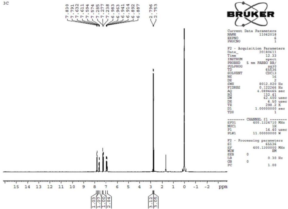
Figure S3: ^1\text{H} -NMR spectrum of ( E )-1-(2',4'-dimethyl)-(5-acetylthiazole)-(2'',4''-difluorophenyl)-prop-2-en-1-one
