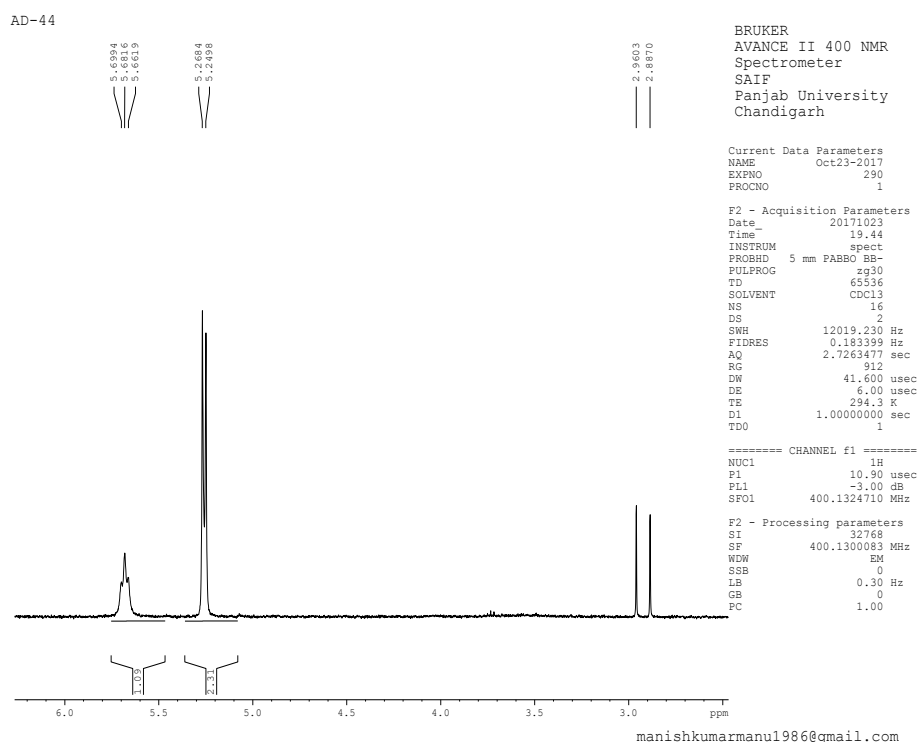
Figure S2c. Extended aliphatic region of ^1\text{H} NMR spectrum of 3-(((2,3-Dichlorophenyl)amino)methyl)-5-(furan-2-ylmethylidene)-1,3-thiazolidine-2,4-dione.
