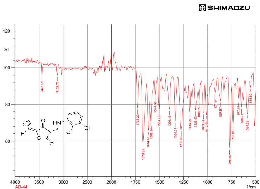
Figure S4. FTIR spectrum of 3-[(2,3-Dichlorophenyl)amino]methyl}-5-(furan-2-ylmethylidene)-1,3-thiazolidine-2,4-dione.
