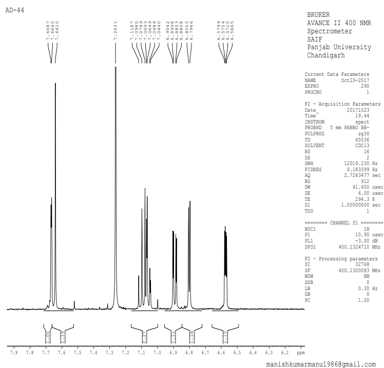
Figure S2b. Extended aromatic region of ^1\text{H} NMR spectrum of 3-(((2,3-Dichlorophenyl)amino)methyl)-5-(furan-2-ylmethylidene)-1,3-thiazolidine-2,4-dione.
