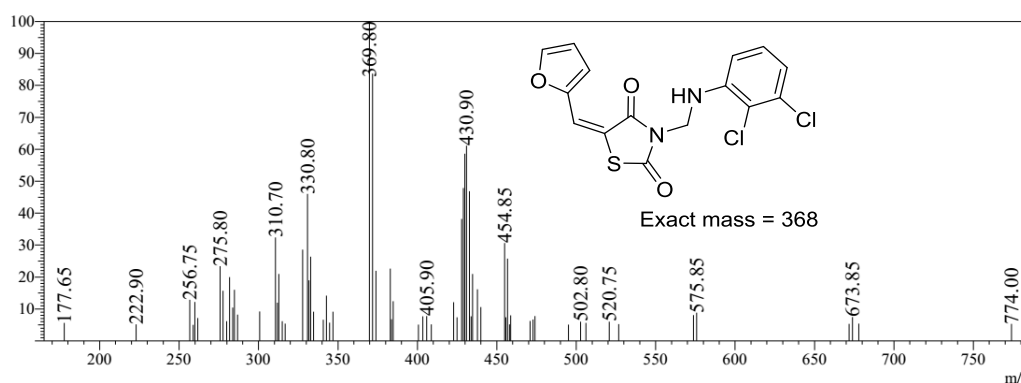
Figure S1. Mass Spectrum of 3-[[[(2,3-Dichlorophenyl)amino]methyl]-5-(furan-2-ylmethylidene)-1,3-thiazolidine-2,4-dione.
