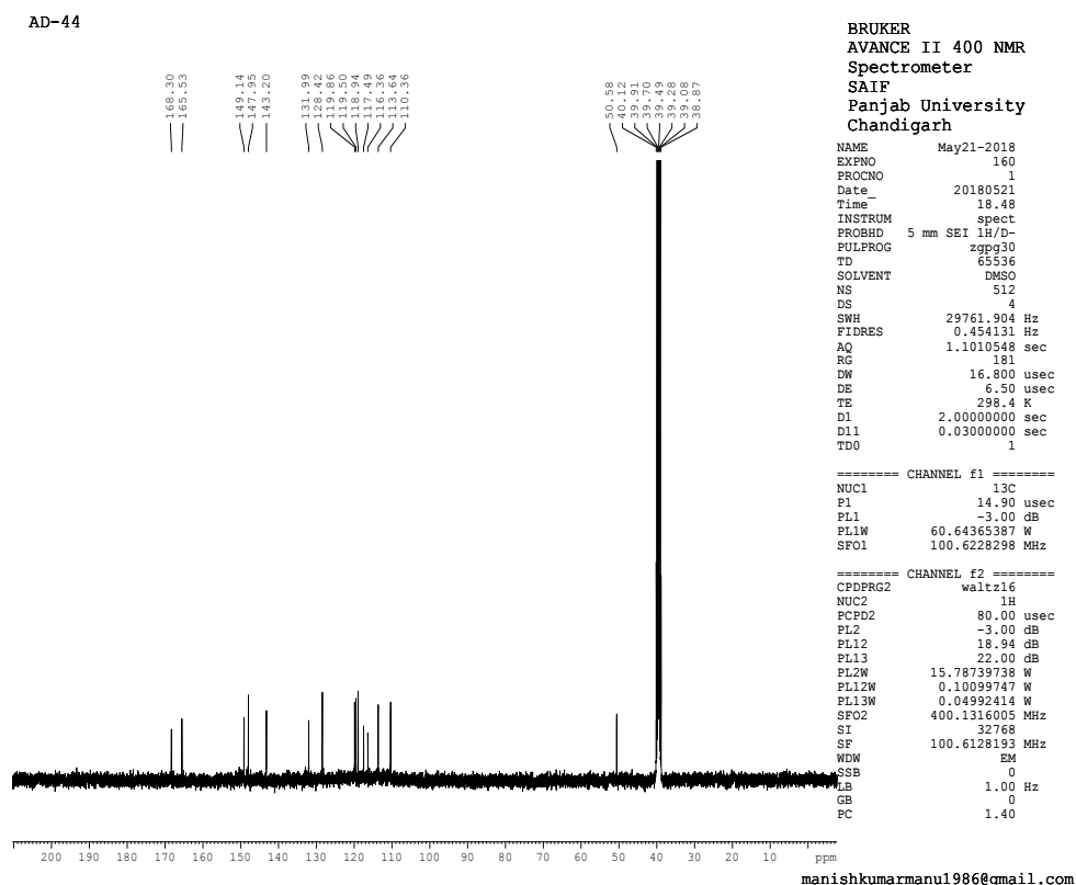
Figure S3. ^{13}\text{C} NMR spectrum of 3-[(2,3-Dichlorophenyl)amino]methyl}-5-(furan-2-ylmethylidene)-1,3-thiazolidine-2,4-dione.
