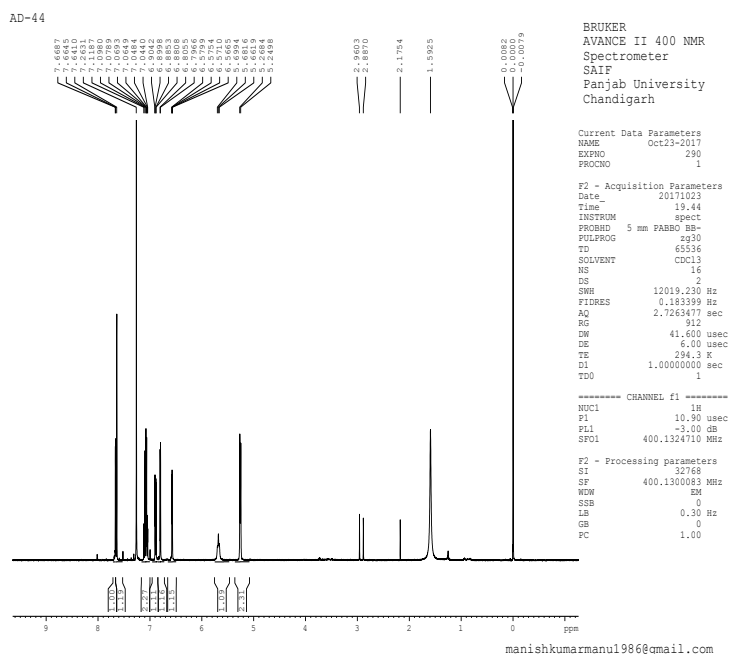
Figure S2a. 1 H NMR spectrum of 3-[[[(2,3-Dichlorophenyl)amino]methyl]-5-(furan-2-ylmethylidene)-1,3-thiazolidine-2,4-dione.
