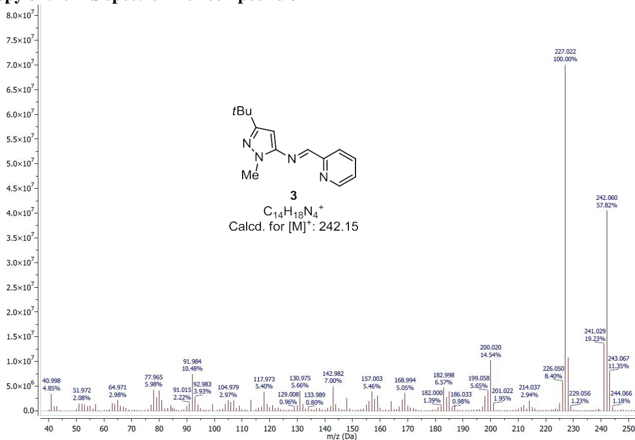
Figure S1. MS spectrum of the compound 3.
