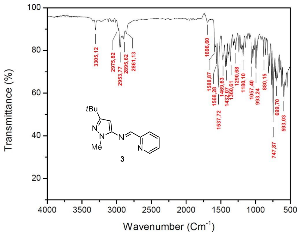
Figure S2. IR spectrum of the compound 3.
