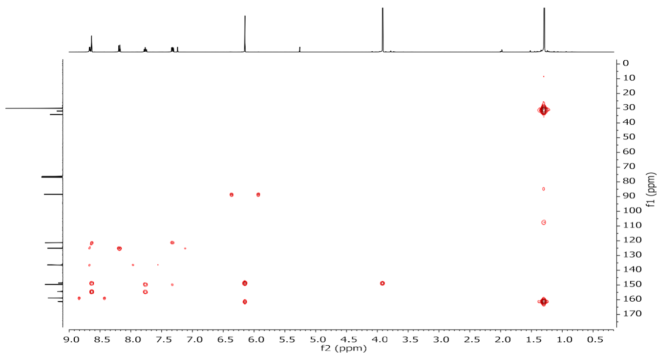
Figure S8. HMBC 2D C-H correlation spectrum of the compound 3.
