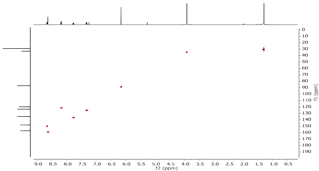
Figure S7. HSQC 2D C-H correlation spectrum of the compound 3.
