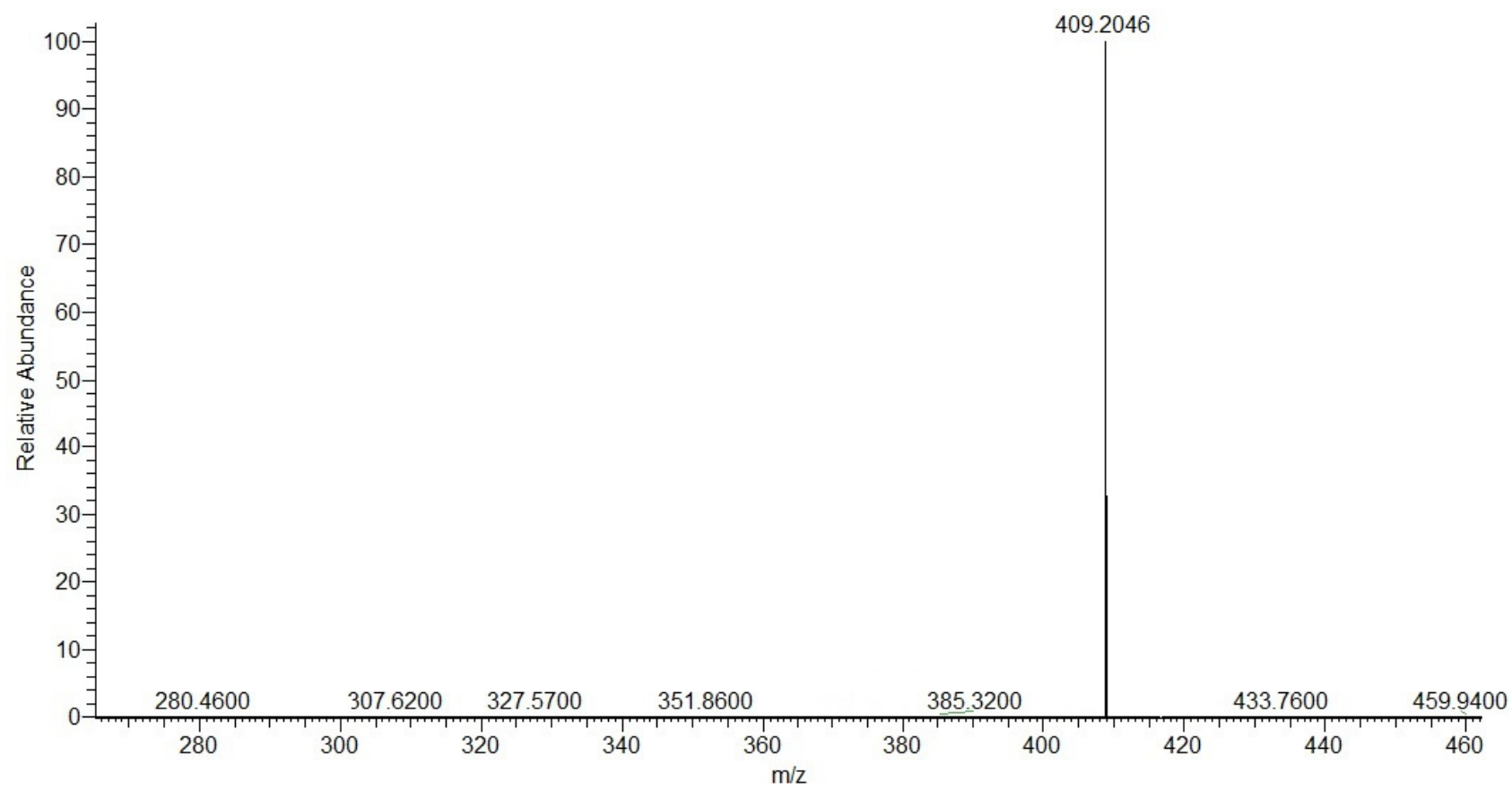
Figure S4. ESI-HRMS of compound 3 .
