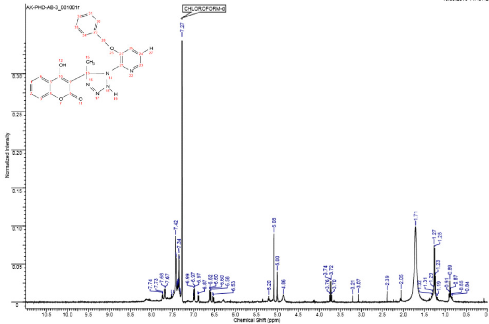
Figure S4. 5d. 3-[1-(3-Benzyloxy-pyridin-2-yl)-5-methyl-2,5-dihydro-1H-tetrazol-5-yl]-4-hydroxy-chromen-2-one
