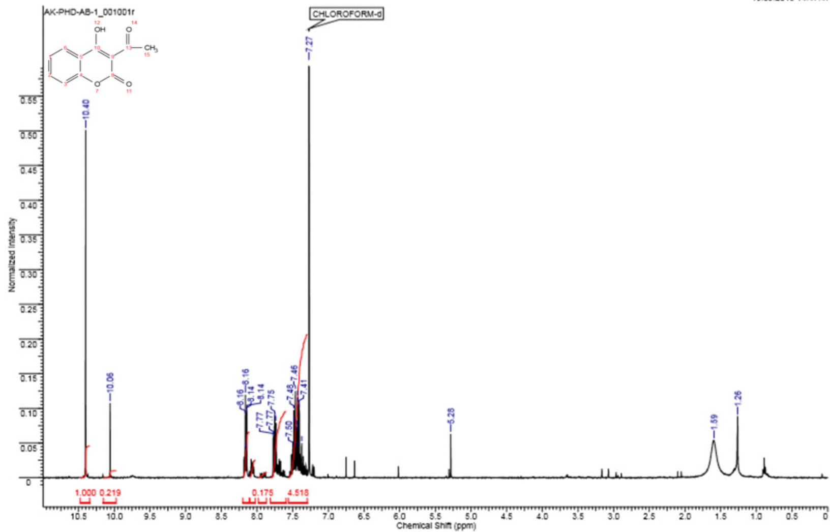
Figure S1. 2. 3-Acetyl-4-hydroxy-chromen-2-one
