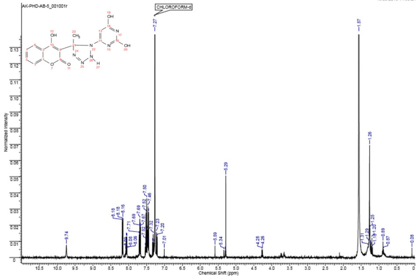
Figure S5. 5e. 3-[1-(2,6-Dihydroxy-pyrimidin-4-yl)-5-methyl-2,5-dihydro-1H-tetrazol-5-yl]-4-hydroxy-chromen-2-one
