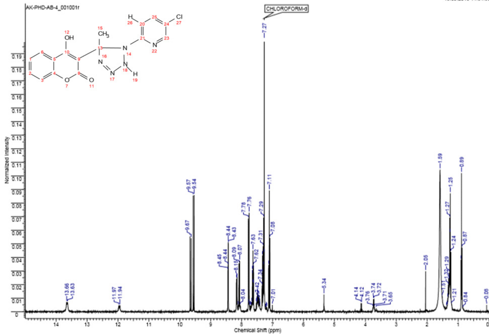
Figure S2. 5a. 3-[1-(5-Chloro-pyridin-2-yl)-5-methyl-2,5-dihydro-1H-tetrazol-5-yl]-4-hydroxy-chromen-2-one
