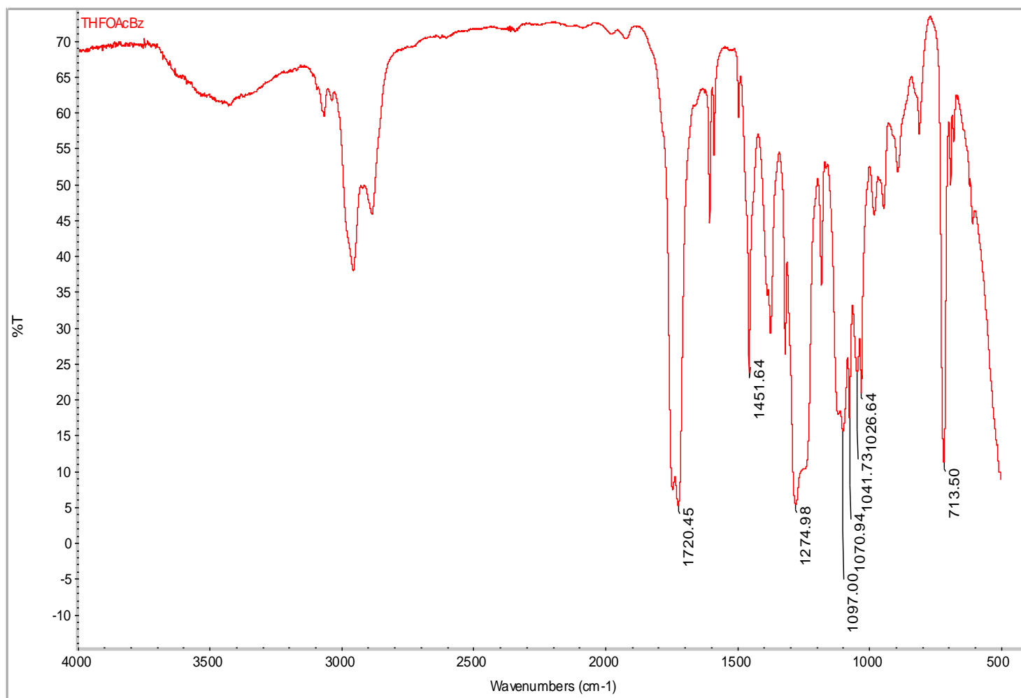
Figure S3. IR spectrum of compound 5.
