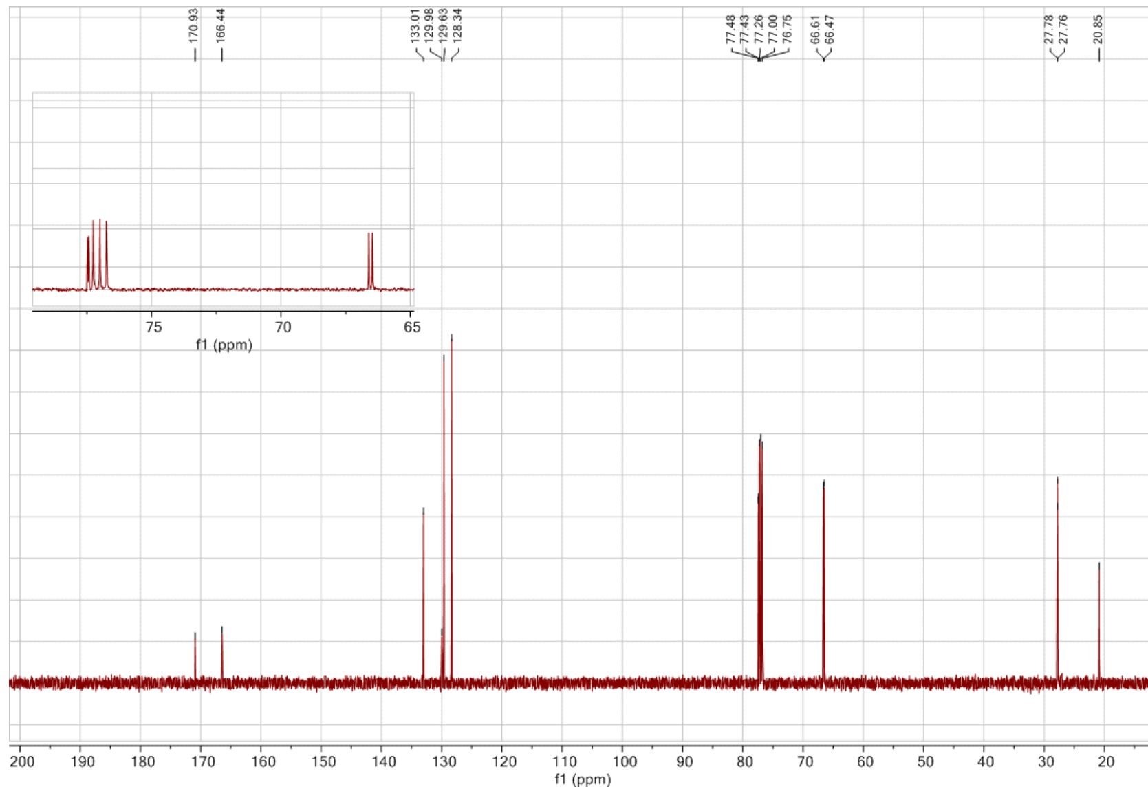
Figure S2. ^{13}\text{C} NMR spectrum of compound 5 ( \text{CDCl}_3 , 100 MHz).
