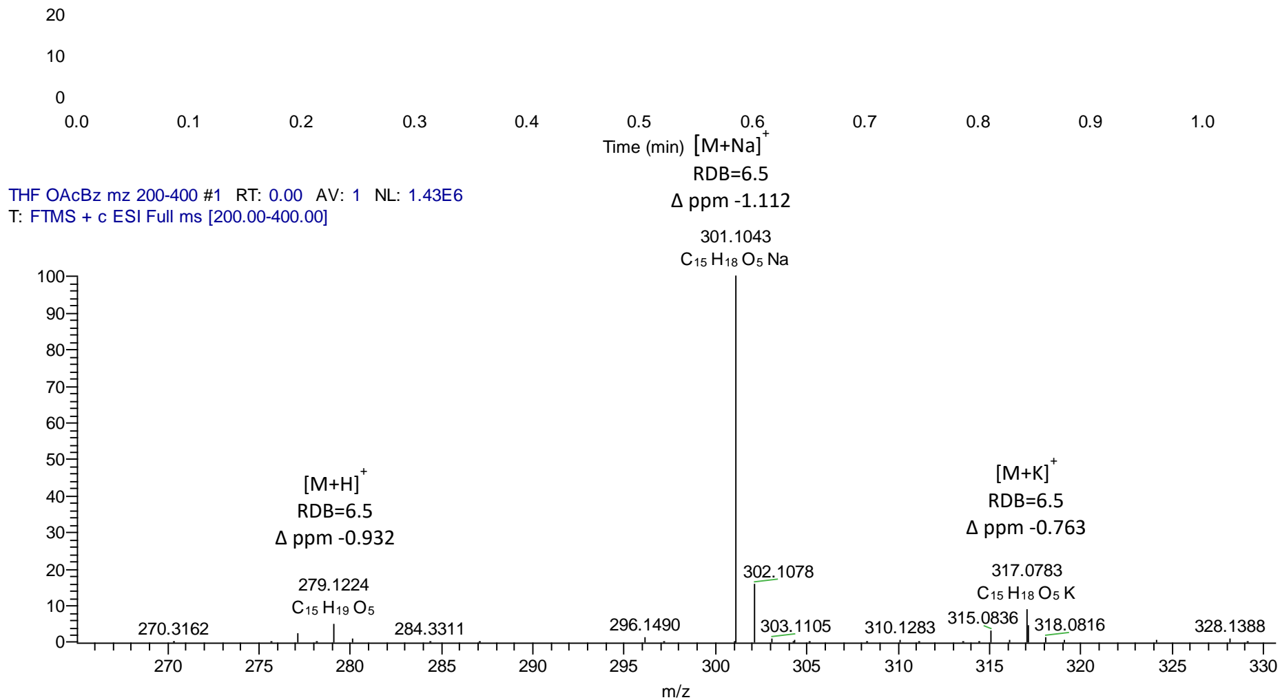
Figure S4. HRESIMS spectrum of compound 5.
