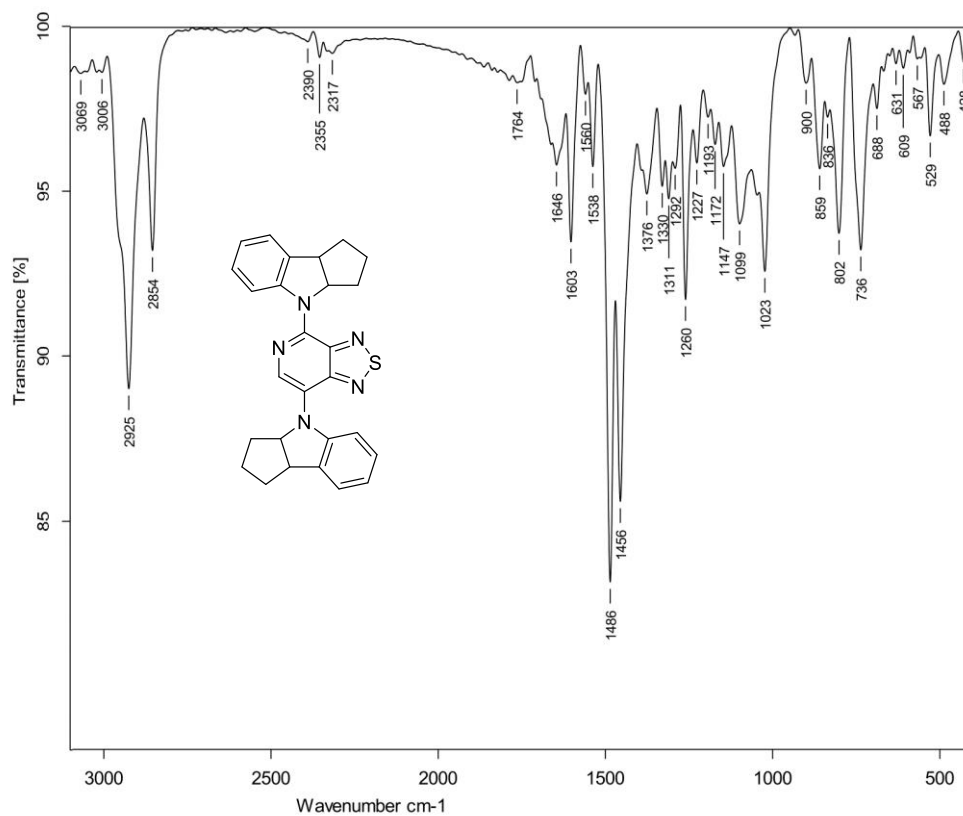
Figure S8. IR spectrum of 4,7-bis(2,3,3a,8b-tetrahydrocyclopenta[ b ]indol-4(1 H )-yl)-[1,2,5]thiadiazolo[3,4- c ]pyridine 1 .
