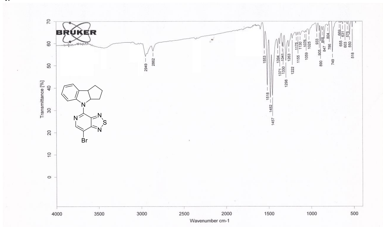
Figure S3. IR spectrum of 7-bromo-4-(2,3,3a,8b-tetrahydrocyclopenta[ b ]indol-4( 1H )-yl)-[1,2,5]thiadiazolo[3,4- c ]pyridine 4.
