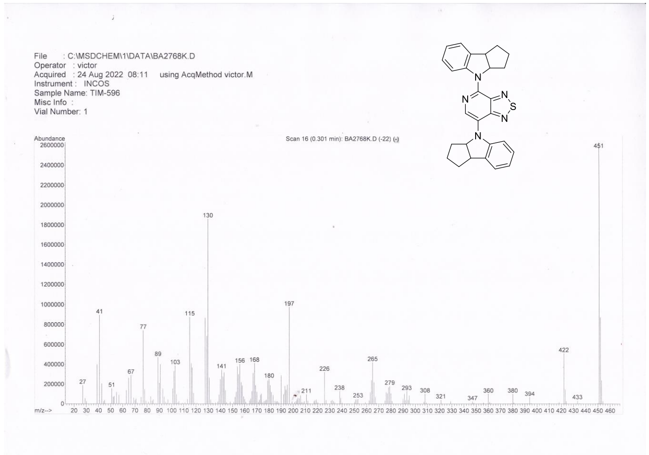
Figure S10. Mass-spectrum of 4,7-bis(2,3,3a,8b-tetrahydrocyclopenta[ b ]indol-4(1 H )-yl)-[1,2,5]thiadiazolo[3,4- c ]pyridine 1 .
