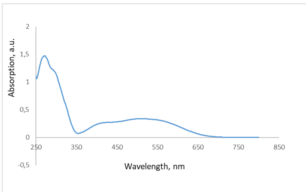
Figure S11. UV-spectrum of 4,7-bis(2,3,3a,8b-tetrahydrocyclopenta[ b ]indol-4(1 H )-yl)-[1,2,5]thiadiazolo[3,4- c ]pyridine 1 .
