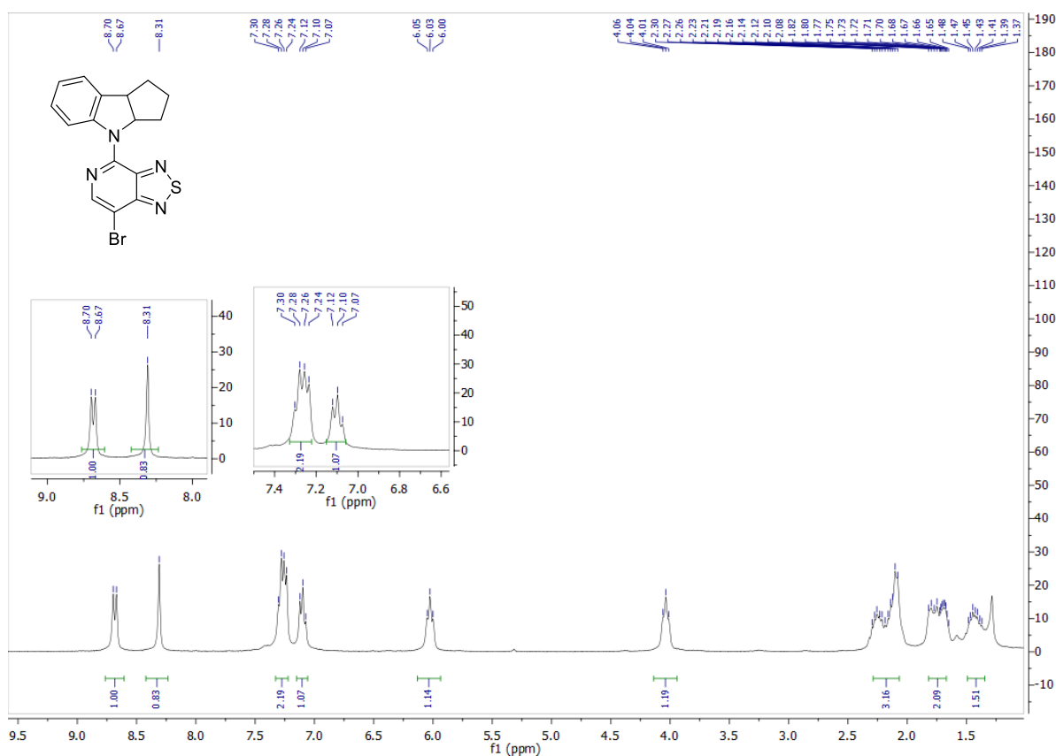
Figure S1. 1 H NMR spectrum of 7-bromo-4-(2,3,3a,8b-tetrahydrocyclopenta[ b ]indol-4(1 H )-yl)-[1,2,5]thiadiazolo[3,4- c ]pyridine 4 .
