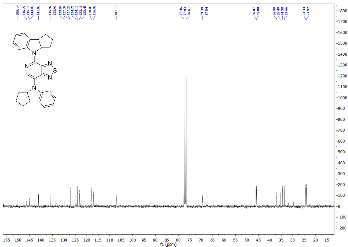
Figure S8. IR spectrum of 4,7-bis(2,3,3a,8b-tetrahydrocyclopenta[ b ]indol-4(1 H )-yl)-[1,2,5]thiadiazolo[3,4- c ]pyridine 1 .
