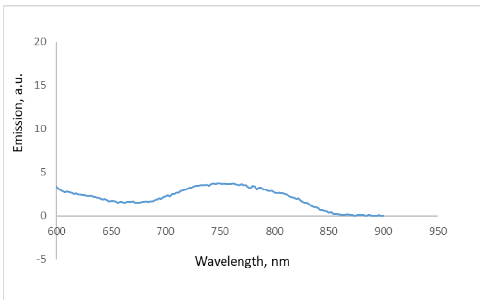
Figure S12. Luminescence-spectrum of 4,7-bis(2,3,3a,8b-tetrahydrocyclopenta[ b ]indol-4(1 H )-yl)-[1,2,5]thiadiazolo[3,4- c ]pyridine 1 .
