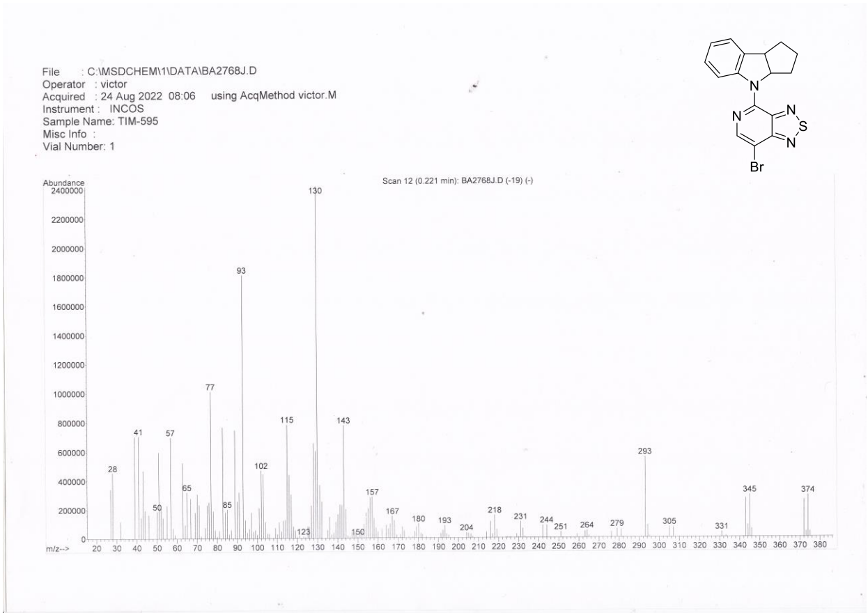
Figure S5. Mass-spectrum of 7-bromo-4-(2,3,3a,8b-tetrahydrocyclopenta[ b ]indol-4(1 H )-yl)-[1,2,5]thiadiazolo[3,4- c ]pyridine 4.
