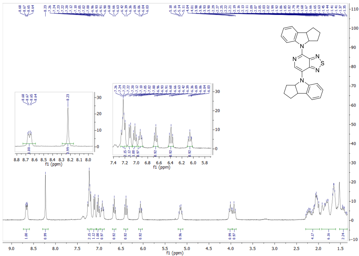
Figure S6. ^1\text{H} NMR spectrum of 4,7-bis(2,3,3a,8b-tetrahydrocyclopenta[ b ]indol-4(1 H )-yl)-[1,2,5]thiadiazolo[3,4- c ]pyridine 1 .
