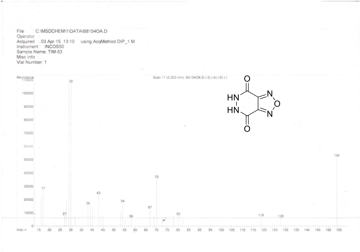
Figure S5. Mass-spectrum of 5,6-dihydro-[1,2,5]oxadiazolo[3,4-d]pyridazine-4,7-dione 1 .
