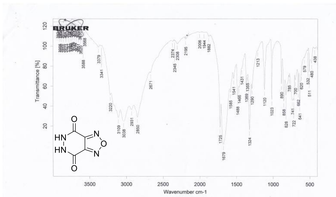
Figure S3. IR spectrum of 5,6-dihydro-[1,2,5]oxadiazolo[3,4-d]pyridazine-4,7-dione 1 .
