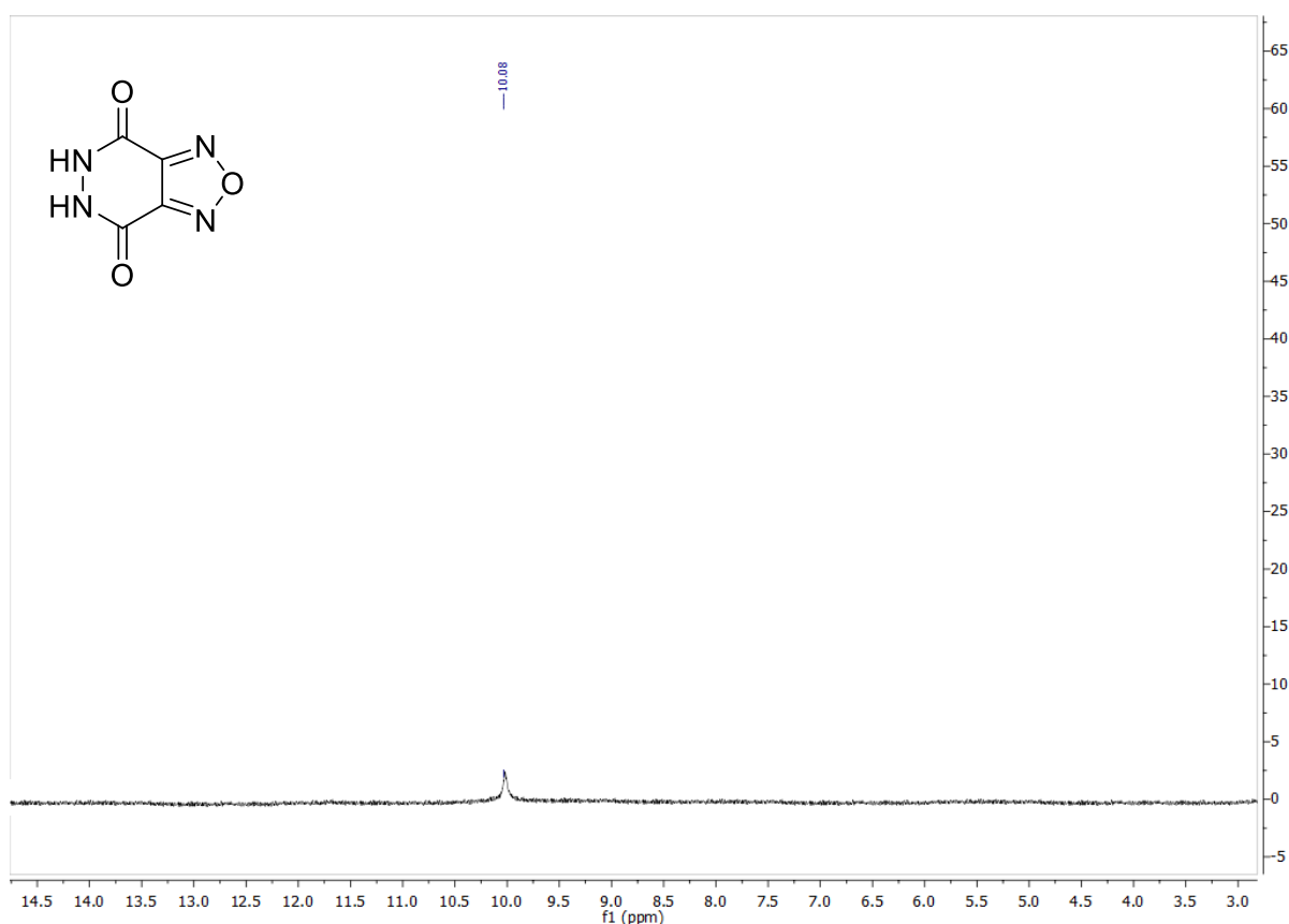
Figure S1. 1 H NMR spectrum of 5,6-dihydro-[1,2,5]oxadiazolo[3,4-d]pyridazine-4,7-dione 1 .
