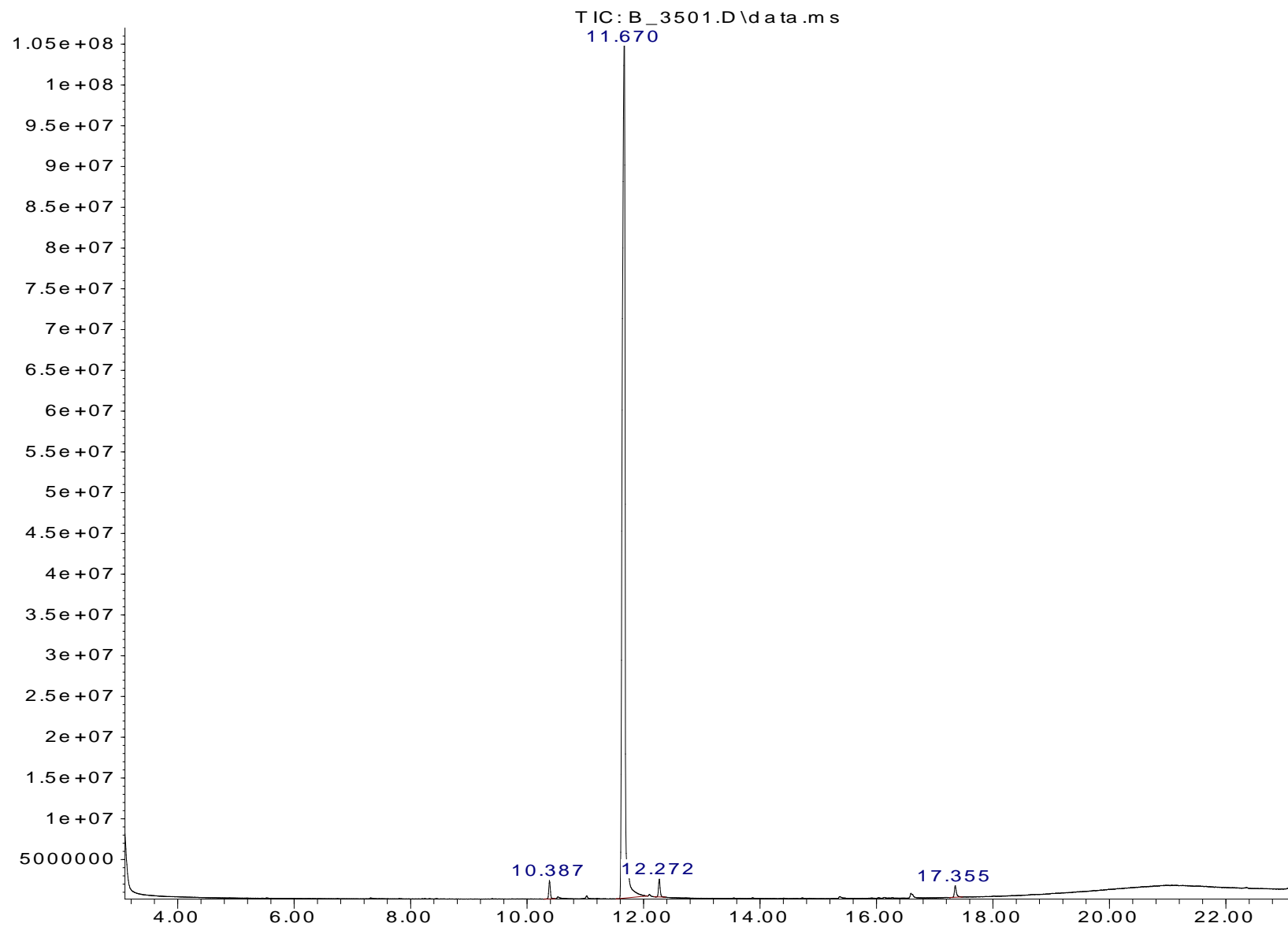
Figure S1. Chromatogram of compound 2
