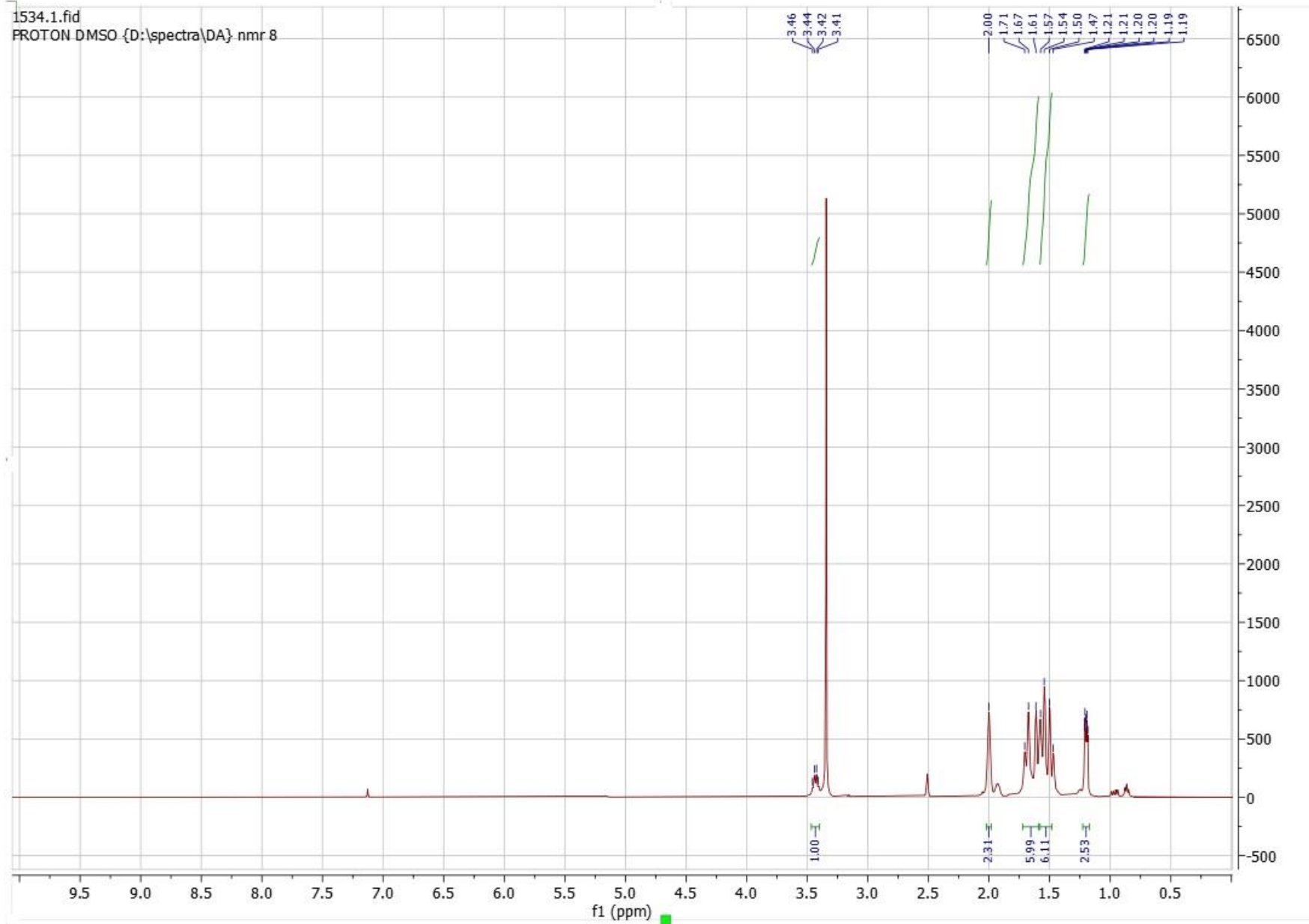
Figure S3. NMR ^1\text{H} of compound 2
