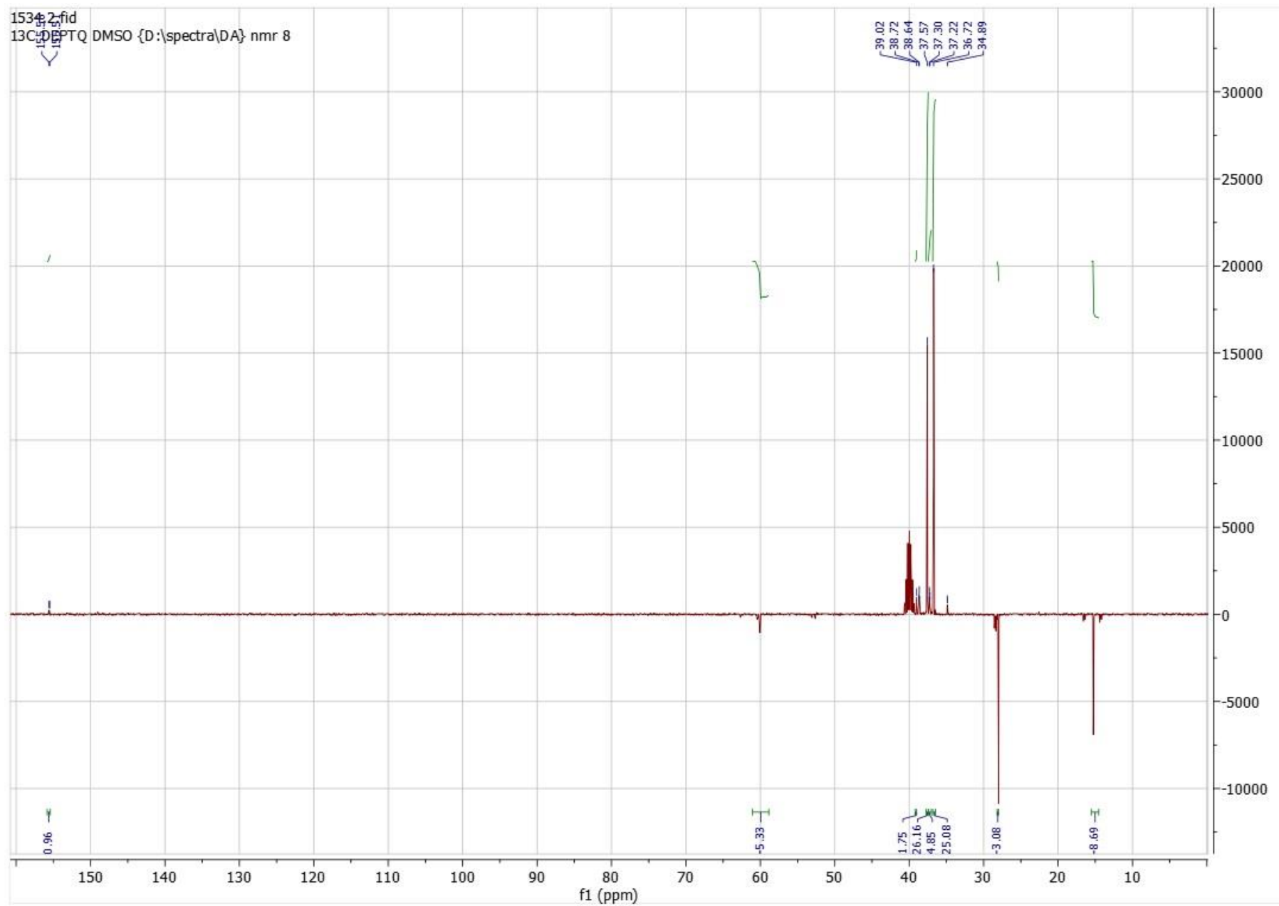
Figure S4. NMR ^{13}\text{C} of compound 2
