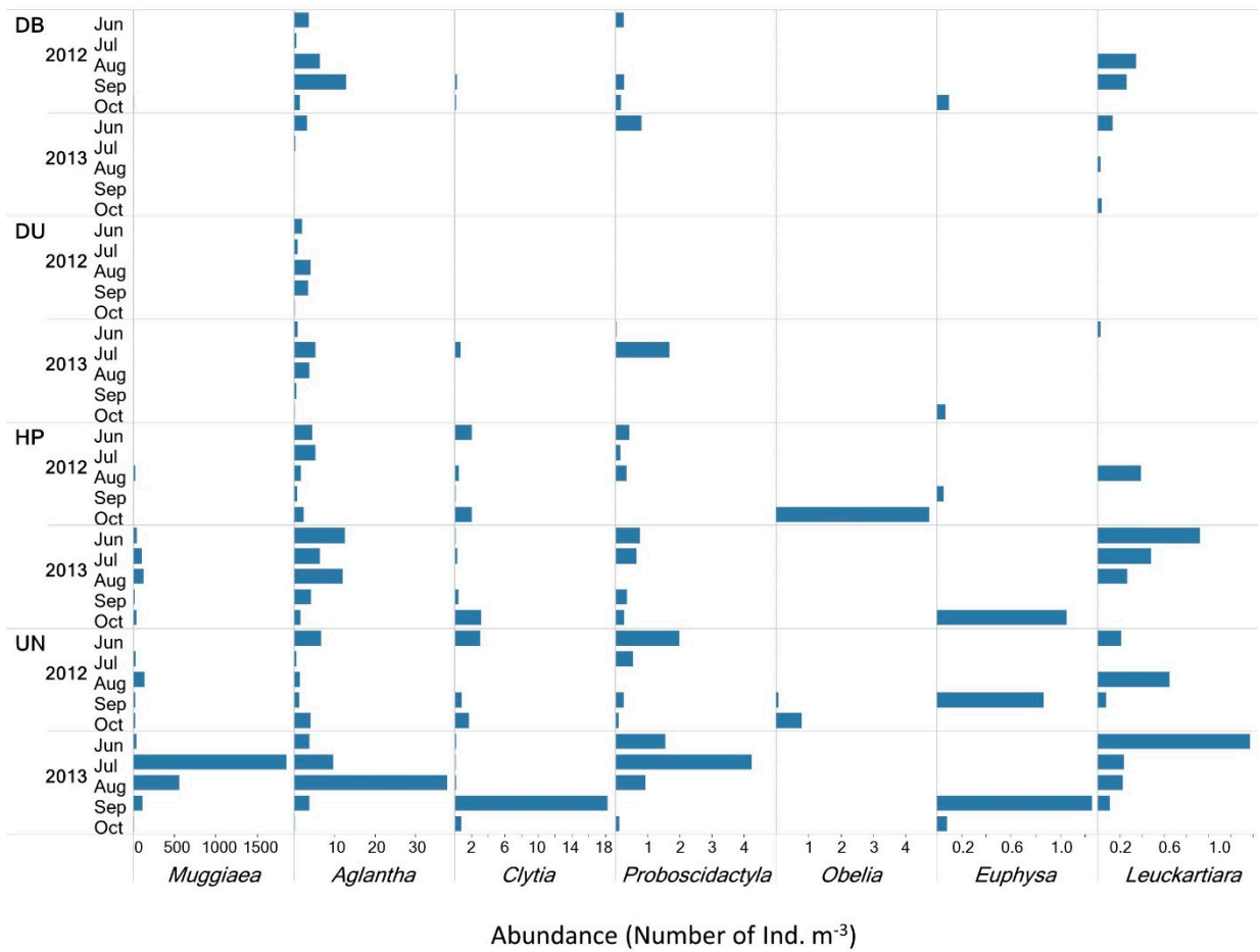
Figure S2. Abundances (number of individuals m -3 ) of dominant gelatinous zooplankton taxa at each station by month and year. Full species names where known are given in the text. See Figure 1 for station abbreviations.
