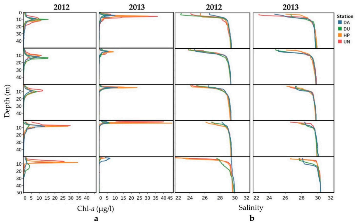
Figure S1. Upper 50-m profiles of (a) chlorophyll and (b) salinity in June through October of 2012 and 2013 from CTD casts conducted at the four sampling sites in Hood Canal.
