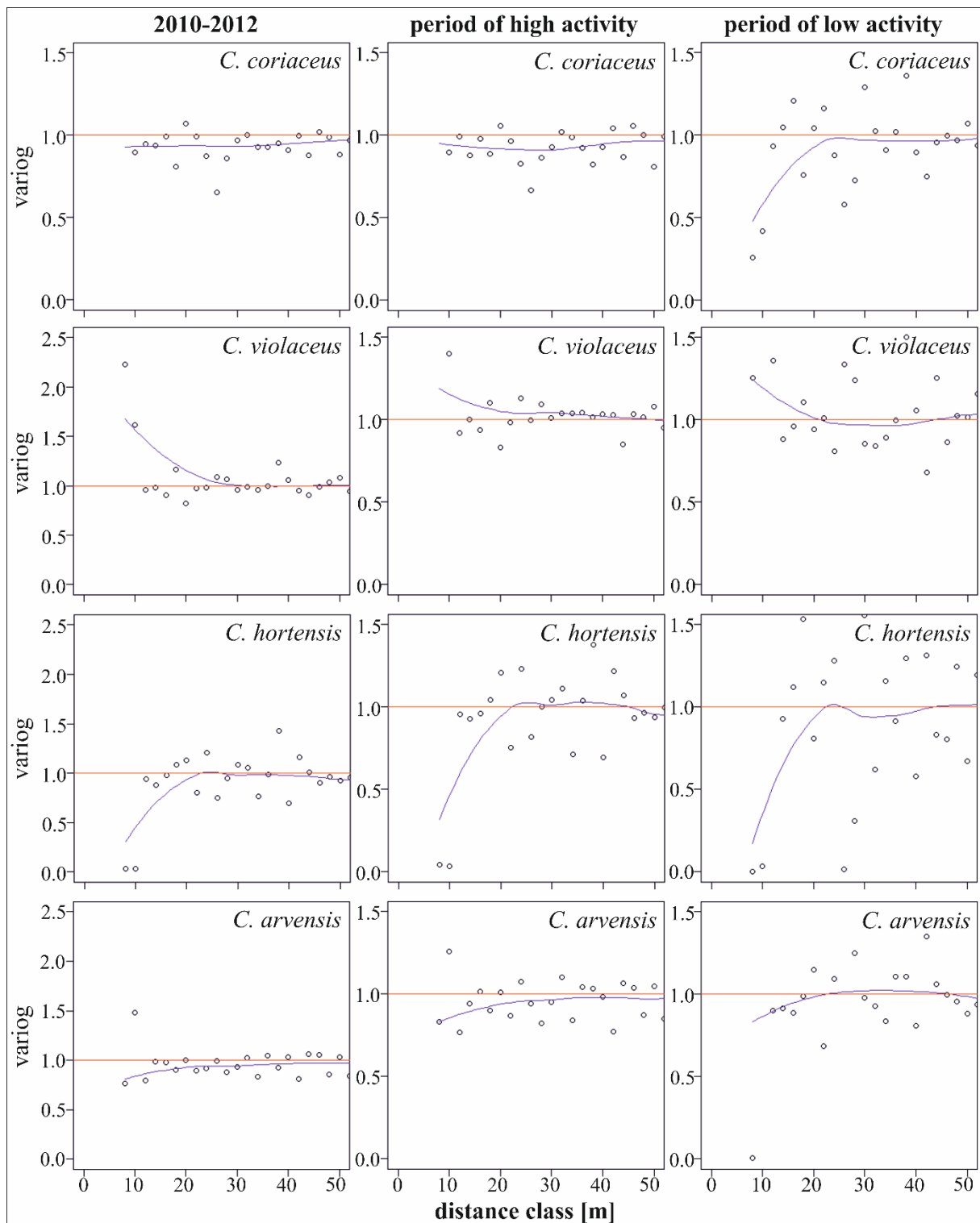
Figure S1. Semi-variograms for testing autocorrelation effects with varying trap distances for intraspecific interactions. The graph of a local polynomial regression is also drawn in. Please note the different y-axes.
