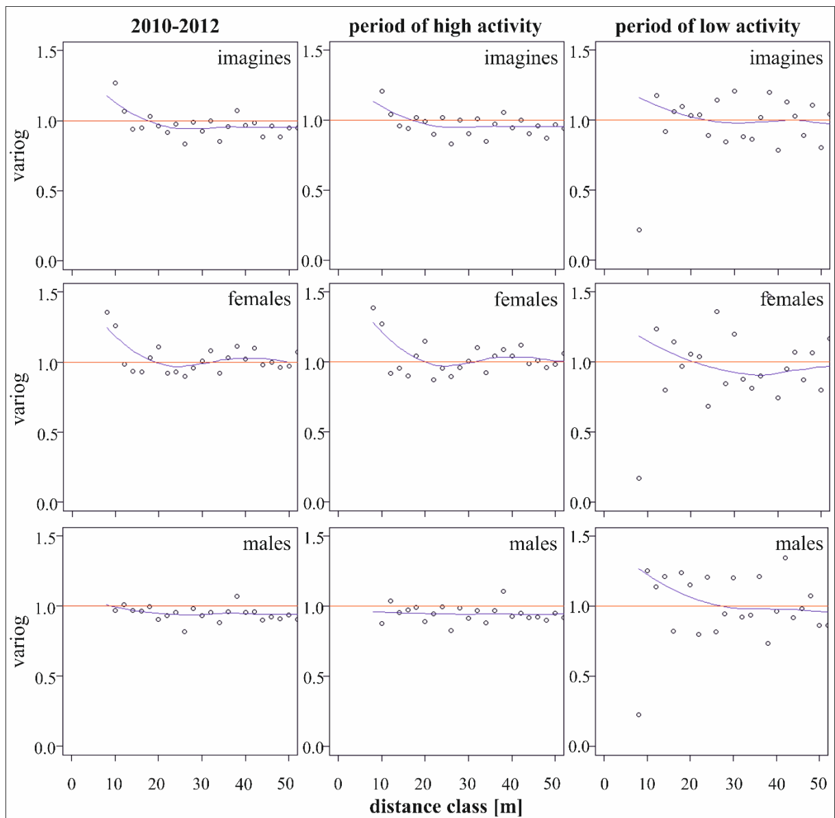
Figure S2. Semi-variograms for testing autocorrelation effects with varying trap distances for interspecific interactions. The graph of a local polynomial regression is also drawn in.
