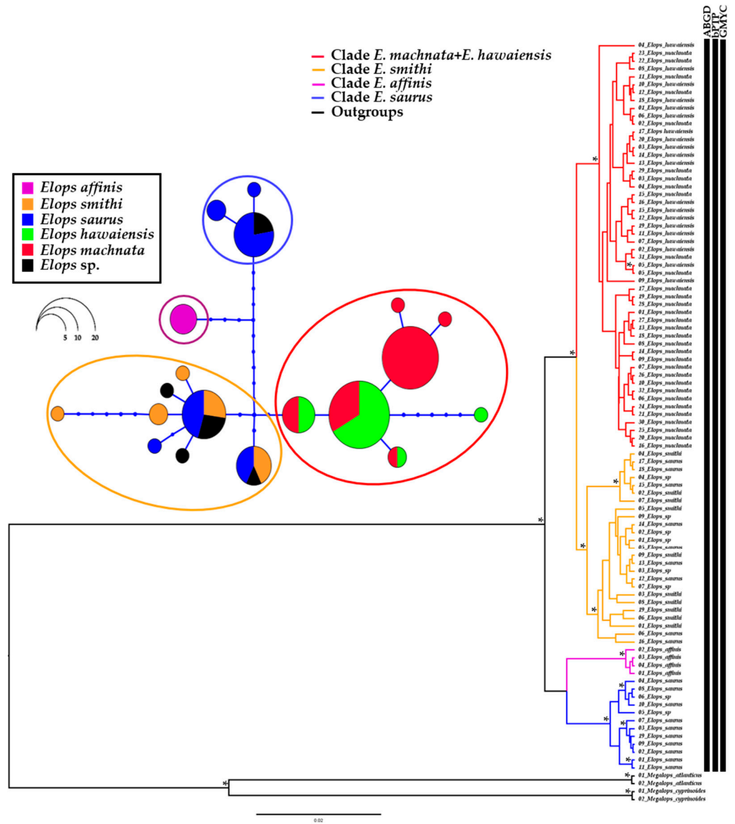
Figure 2. Ultrametric tree and haplotype network representing the relationships of Elops species. In the network, each circle represents one haplotype, and the size of the circles is proportional to the haplotype frequency. Color codes represent the species, and the color codes in line of the ultrametric tree represent the clades found in Elops species. Vertical bars (on the right) indicate the results of the delimitation analysis based on ABGD, bPTP, and GMYC, respectively. Asterisks (*) at nodes indicate posterior probability > 0.9.
