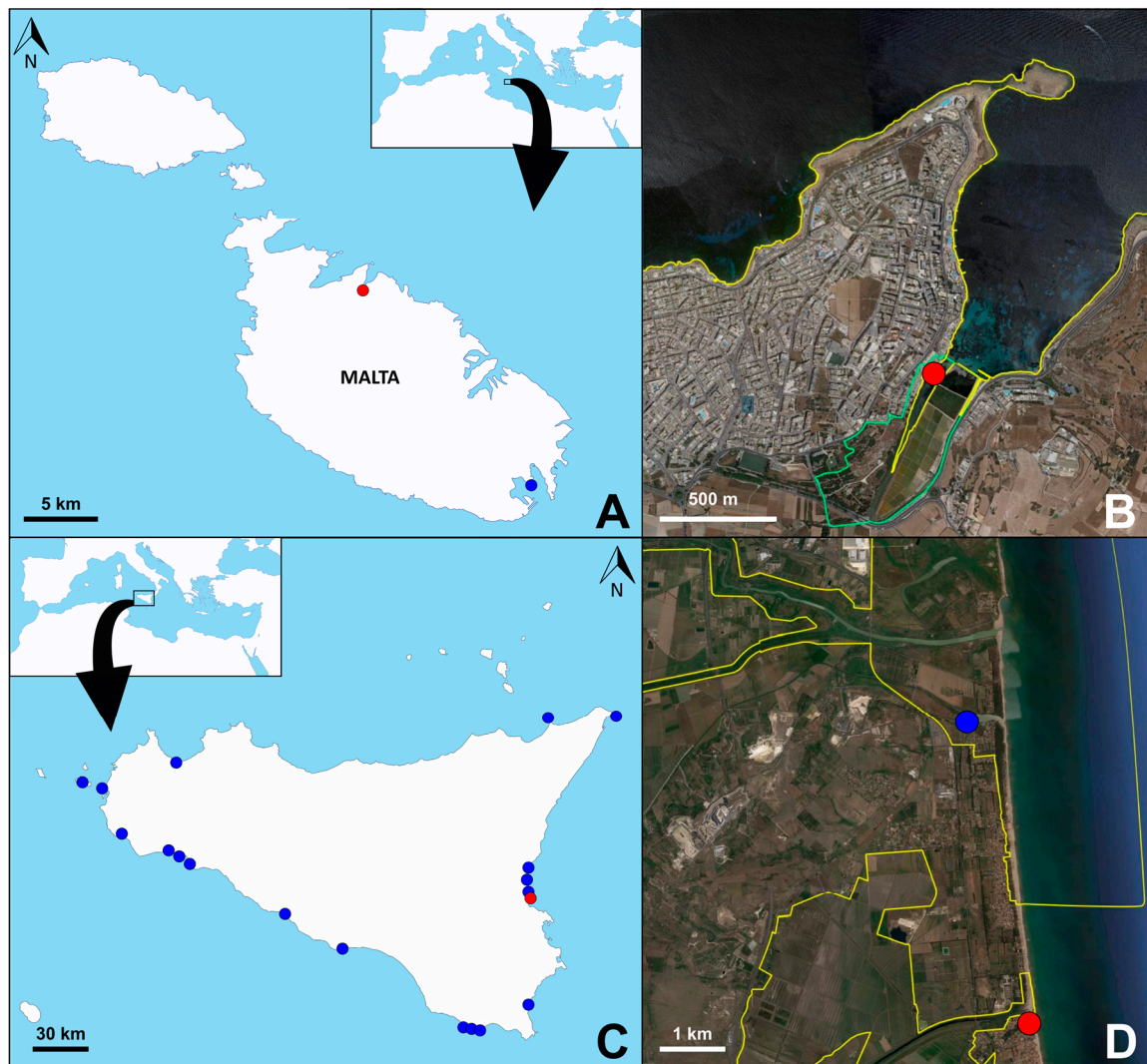
Figure 1. (A) Map of Malta showing the 2020 record (red) and the 2021 record (blue [30]); (B) map of the Is-Salini area, Malta showing the location of the current new record (red), including the outlines of the Natura 2000 sites MT0000007 (green) and MT0000112 (yellow); (C) map of Sicily showing the current record (red) and previous records (blue [20]); (D) map of the San Leonardo River estuary, Sicily showing the location of a previous record (blue) and current record (red), including the outline of the Natura 2000 site ITA070029 (yellow). (Source: http://www.google.com/earth/index.html and https://natura2000.eea.europa.eu (accessed on 7 April 2023)).
