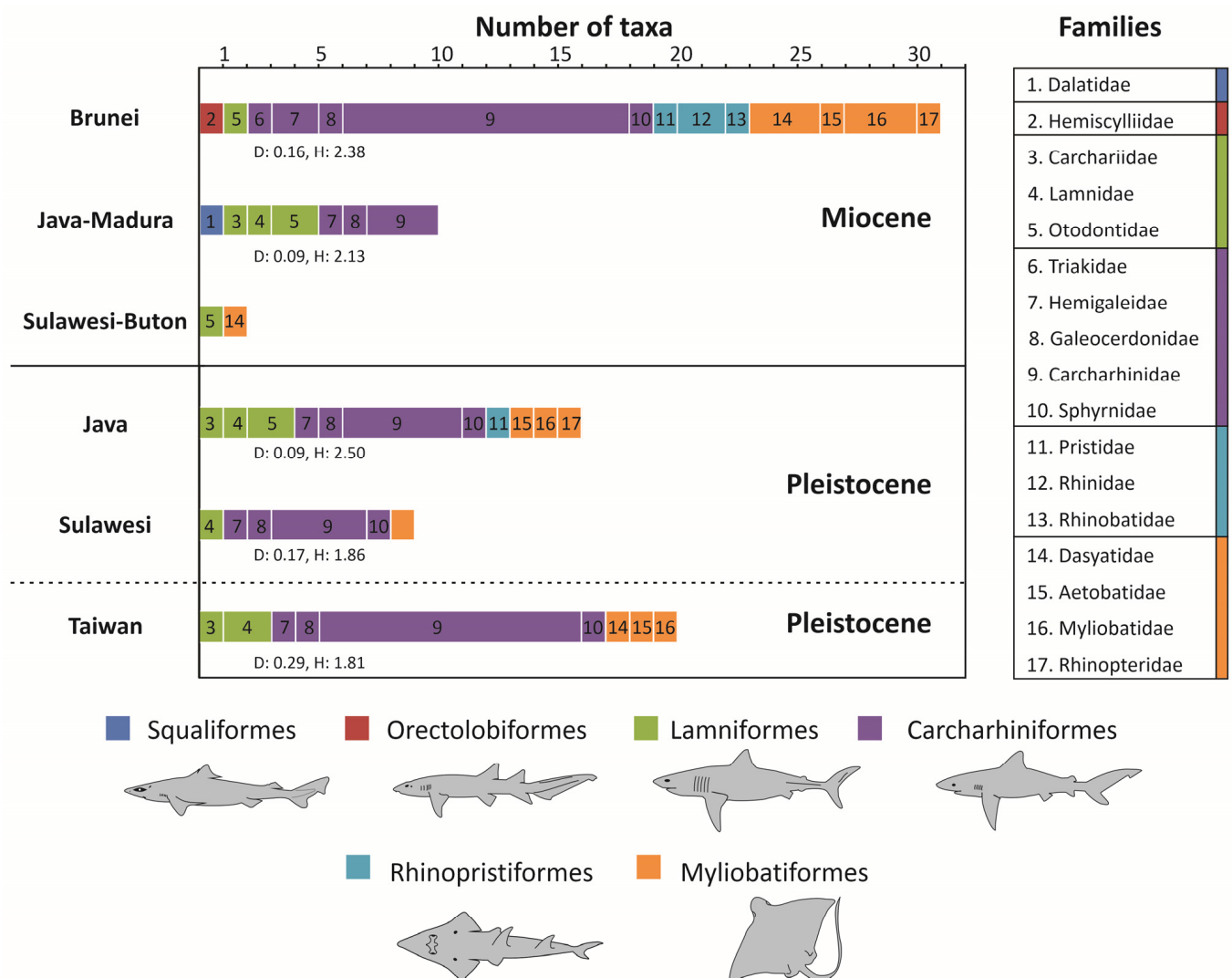
Figure 9. Comparative chart of the presence of different elasmobranch taxa in the Indo-Australian Archipelago during the Miocene and the Pleistocene (see also Tables 1 and 2). Data from recently published revised Pleistocene elasmobranch fauna from Taiwan, situated just north of South China Sea and the IAA, are also included [71]. Note that sporadic occurrences are not illustrated here (Sumatra, Timor, see Table 2). Diversity indices based on number of taxa within the families are shown below the bars: D–Dominance and H–Shannon index.
