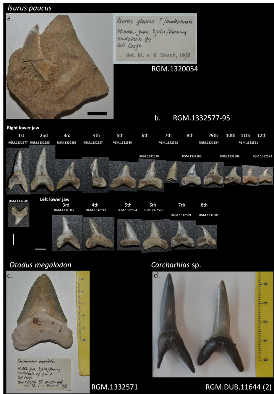
Figure A4. (a) Isurus paucus (RGM.1320054), early Pleistocene, Jetis, Java. Scale bar 1 cm. (b) Tooth series of Isurus paucus (RGM.1332577–95). There are 27 teeth (26 lower and 1 upper) that belong to the same individual. All of the teeth are in lingual views. There was no indication of locality in the RGM collection, but they were together with Cosijn's specimens from Jetis. The teeth have similar size, preservation, and partly coloration as the teeth in the block from Jetis above (C4.1). Therefore, they may derive from the same fossil shark specimen. Scale bar 1 cm. (c) Otodus megalodon (RGM.1332571) early Pleistocene, Jetis, Java. Note that the taxon is considered to have become extinct by the Pleistocene. Therefore, either this specimen represents the youngest occurrence of this species or the age of the locality and/or origin of the tooth need to be further investigated. (d) Carcharias sp. (RGM.DUB.11644) middle Pleistocene, Trinil, Java. Note that these teeth have been described as Odontaspis cuspidata , which corresponds to Araloselachus cuspidatus based on modern nomenclature [45]. However, this latter taxon has teeth with smooth enameloid on the lingual face of the crown, but the crown of the Trinil teeth bear fine striation.
