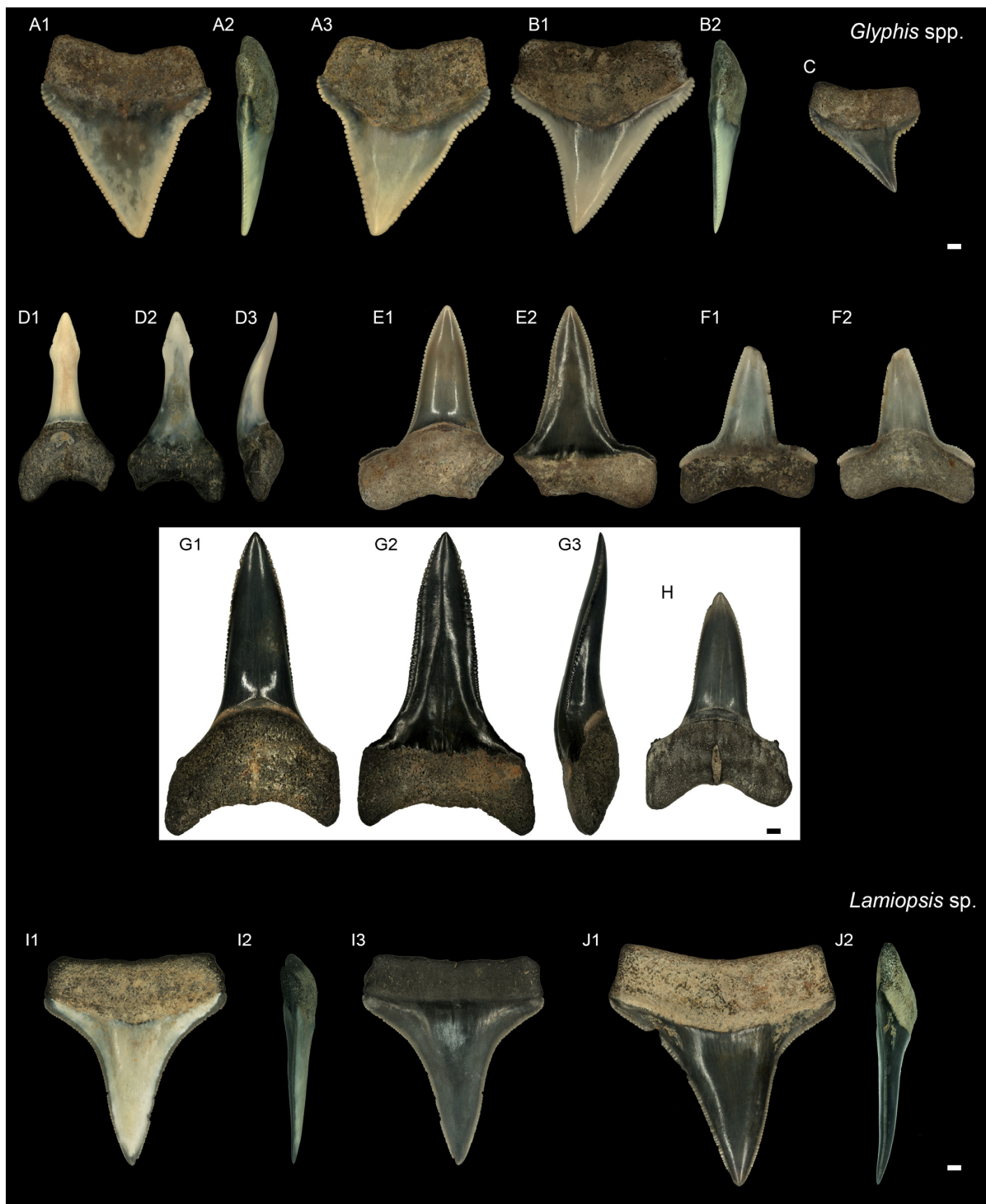
Figure 7. (A–H). Glyphis spp. (A) Upper anterior (Ker: GUBD V0259a). (A1) Labial, (A2) lateral, and (A3) lingual views. (B) Upper anterolateral. (B1) Lingual and (B2) lateral views (Ker: GUBD V0259b). (C) Upper lateral in lingual view (Ker: GUBD V0260). (D) Lower anterior. (D1) Lingual, (D2) labial, and (D3) lateral views (JPB: GUBD V0263). (E) Lower anterolateral. (E1) Lingual and (E2) labial views (Ker: GUBD V0261a). (F) Lower anterolateral. (F1) Lingual and (F2) labial views (Ker: GUBD V0261b). (G) Lower anterior. (G1) Lingual, (G2) labial, and (G3) lateral views (JPB: GUBD V0262a). (H) Lower anterior in lingual view (JPB: GUBD V0262b). (I,J) Lamiopsis sp. (JPB: GUBD V0264). (I) Upper anterolateral. (I1) Labial, (I2) lateral, and (I3) lingual views (JPB). (J) Upper anterolateral. (J1) Lingual and (J2) lateral views (JPB). Scale bars 1 mm.
