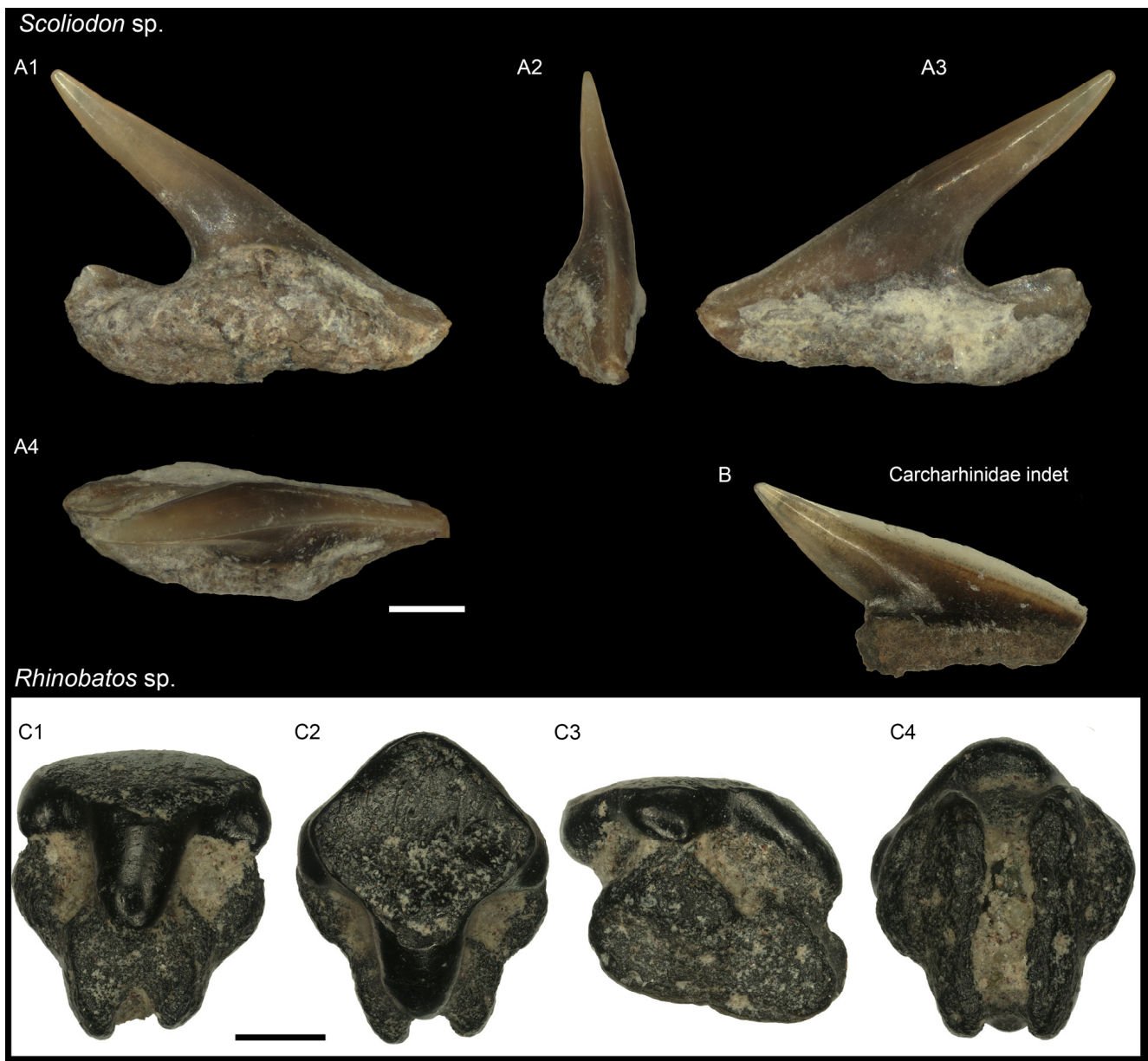
Figure 8. (A) Scoliodon sp. (Ker: GUBD V0265). (A1) Lingual, (A2) lateral (mesial), (A3) labial, and (A4) apical views. (B) Carcharhinidae indet, lingual view, note that such a crown shape can be related to Scoliodon , Loxodon , or Rhizoprionodon genera. (C) Rhinobatidae , Rhinobatos sp. (JPB: GUBD V0266). (C1) Lingual, (C2) occlusal/apical, (C3) lateral, and (C4) basal views (JPB). Scale bars 0.5 mm.
