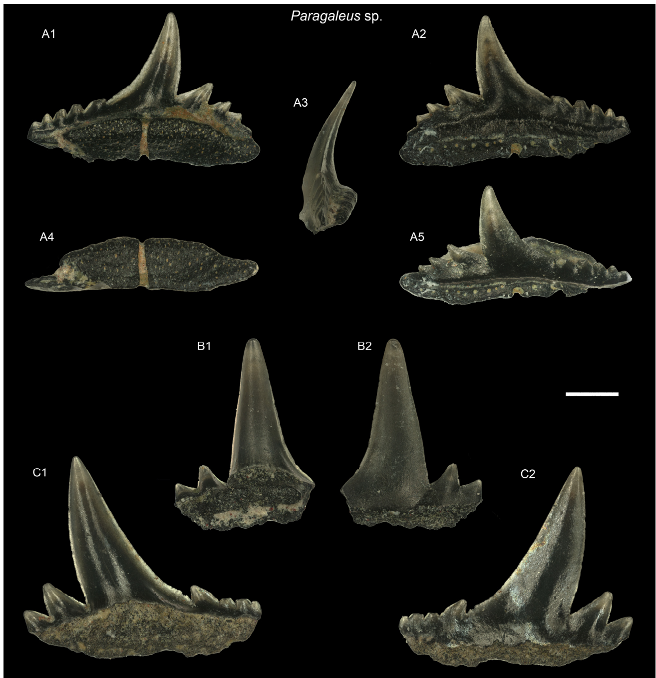
Figure 4. (A–C) Paragaleus sp. teeth (JPB: GUBD V0253). (A) Lateral tooth, (A1) lingual, (A2) labial, (A3) lateral (mesial), (A4) basal, and (A5) apicolabial views. (B) Anterior tooth, (B1) lingual and (B2) labial views. (C) Lateral tooth, (C1) lingual, and (C2) labial views. Scale bar 0.5 mm.
