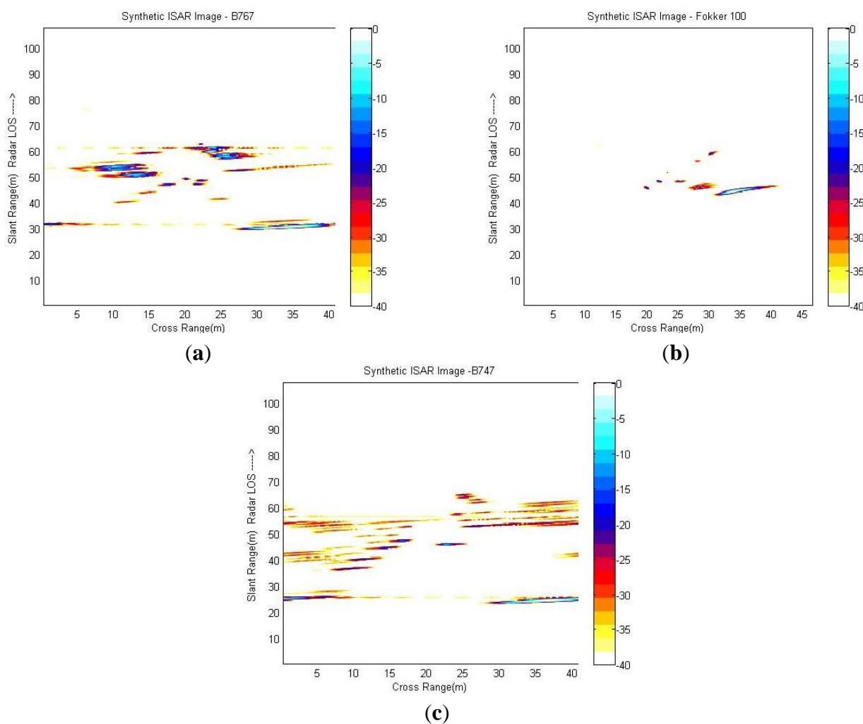
Figure 11. Examples of ISAR images populating the synthetic database; (a) Synthetic ISAR image of a Boeing 767; (b) Synthetic ISAR image of a Fokker 100; (c) Synthetic ISAR image of a Boeing 747.
