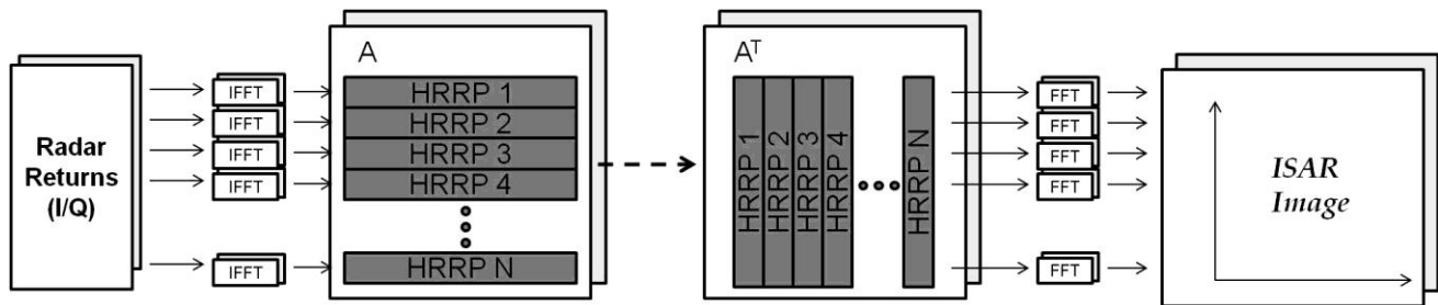
Figure 5. RDA Algorithm.
