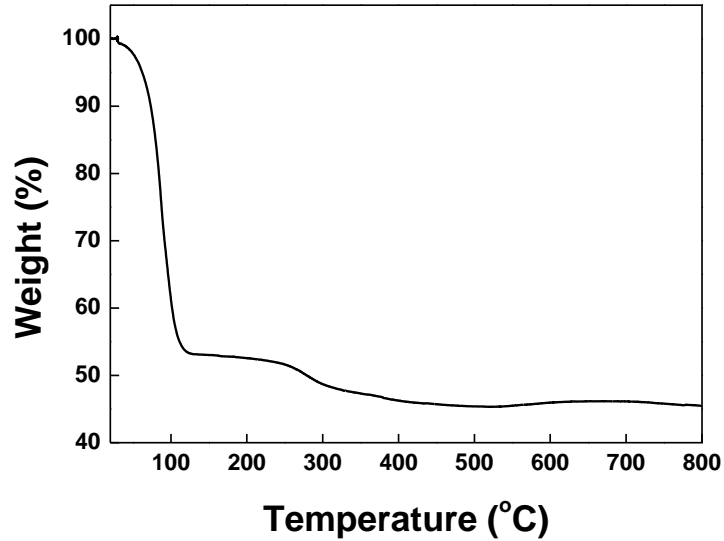
Figure S1: Thermo-gravimetric analysis (TGA) graph of the nickel/carbon composites at a 10 °C/min ramp rate.
