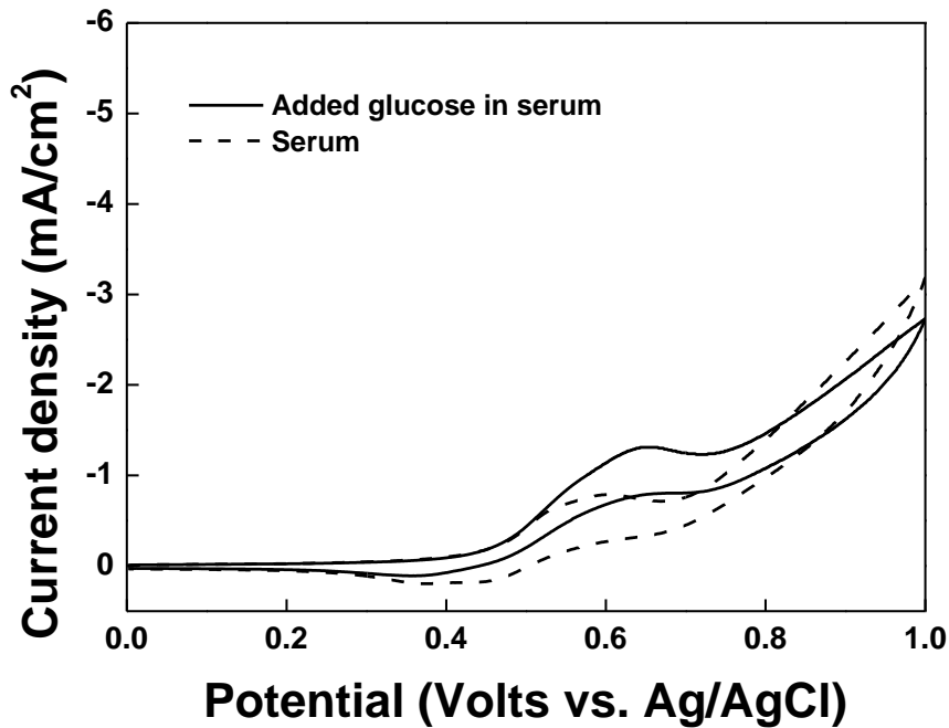
Figure S2: Cyclic voltammograms of added glucose in serum (line) and serum (dot) sample.
