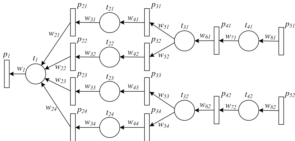
Figure 7. An example of TPN model for a typical manufacturing process.
