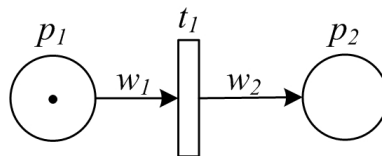
Figure 2. PPN model of sequence pattern.
