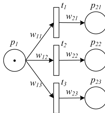
Figure 5. PPN model of exclusive choice pattern.
