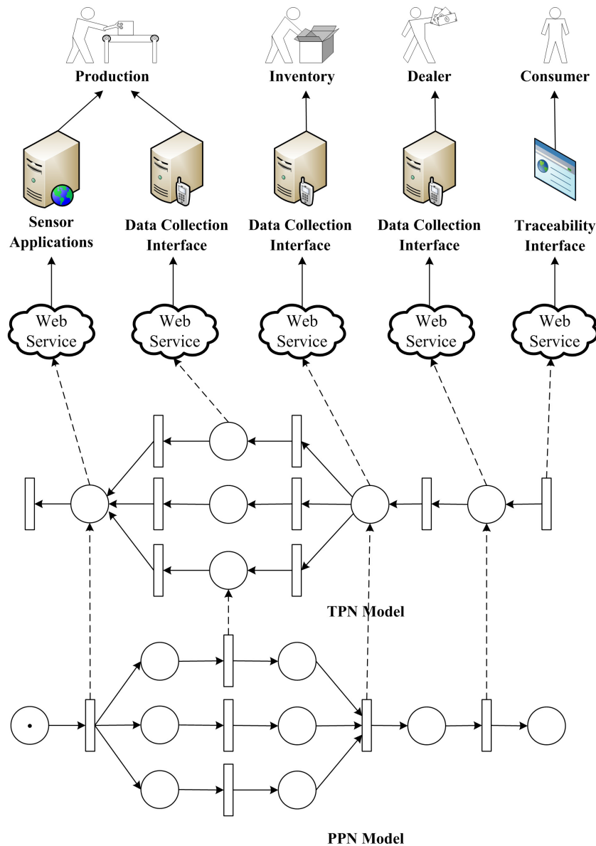
Figure 8. Framework of a traceability solution for cyber-physical manufacturing systems.
