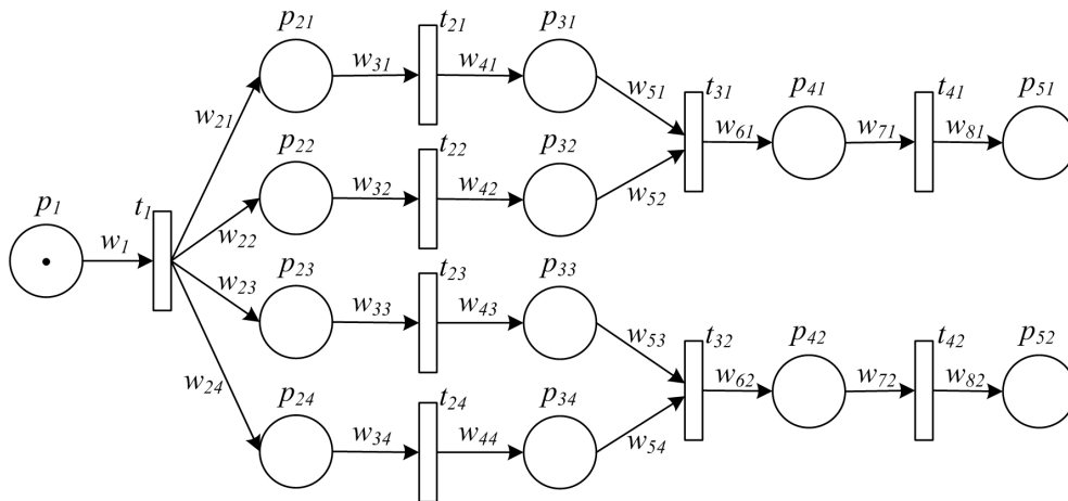
Figure 1. An example of PPN model for a typical manufacturing process.
