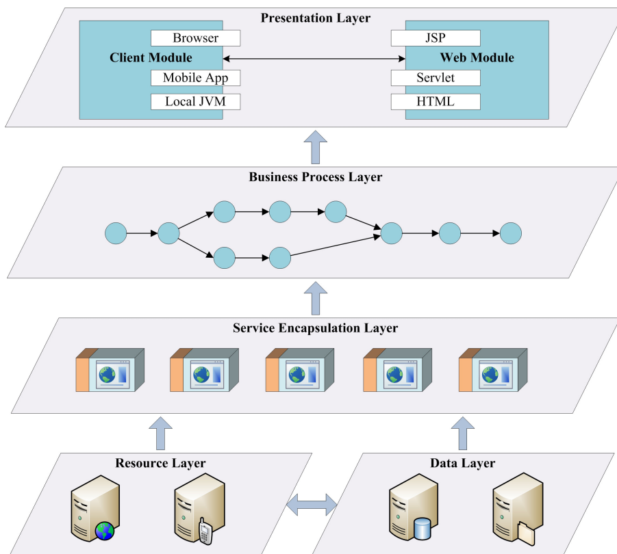
Figure 9. Framework of web service encapsulation.
