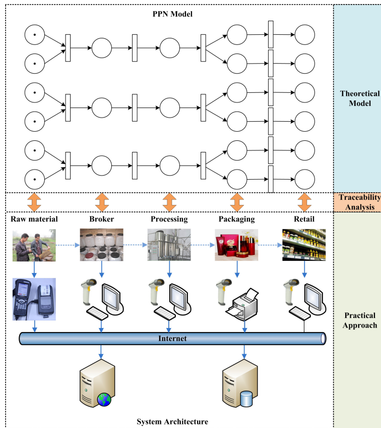
Figure 10. Framework of quality control system for bee products.
