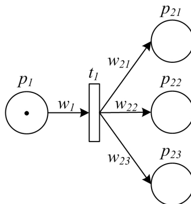
Figure 3. PPN model of split pattern.
