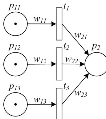
Figure 6. PPN model of simple merge pattern.
