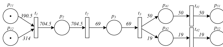
Figure 12. PPN model of the manufacturing process of an orange honey product.
