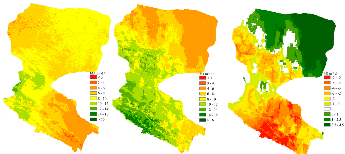
Figure 4. Spatial distribution of daily net radiation ( \text{MJ}\cdot\text{m}^{-2}\cdot\text{d}^{-1} ) estimated using sunshine duration-IDW (left); the proposed model (middle) and the difference between both methods (right) over the Heihe River Basin in 16 July 2008.
