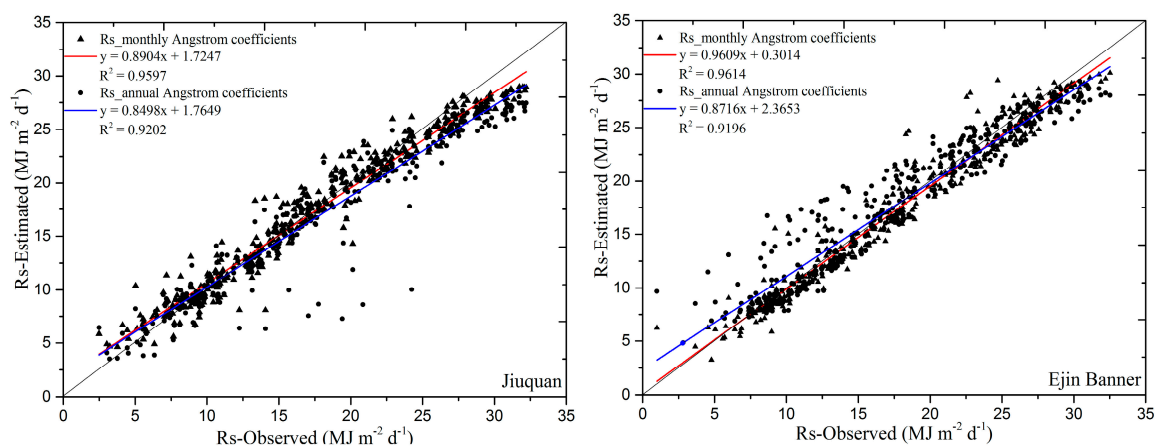
Figure 2. Comparison of the observed and estimated global daily solar radiation in 2008 (366 days) at Jiuquan (left) and Ejn Banner (right).
