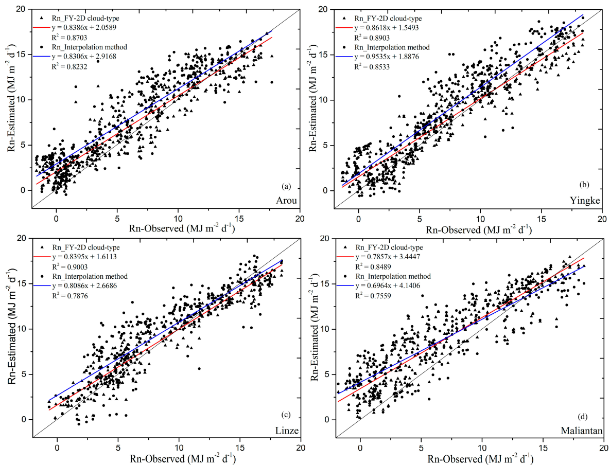
Figure 3. Comparison of the observed and estimated daily net radiation in 2008 (366 days) at Arou (a); Yingke (b) Linze (c) and Maliantan (d) stations.
