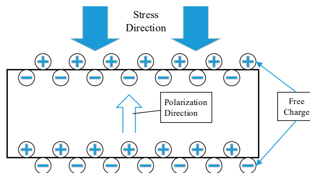
Figure 5. Schematic diagram of the piezoelectric effect.
