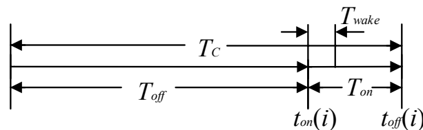
Figure 17. The opening and closing cycles of the sensing system.
