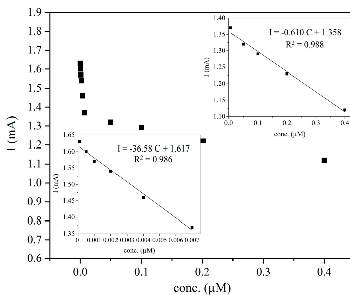
Figure 5. Calibration curve obtained for the developed sensor; (insets are showing two linear ranges of histamine, 1 \times 10^{-10} – 7 \times 10^{-9} M and 7 \times 10^{-9} – 4 \times 10^{-7} M).
