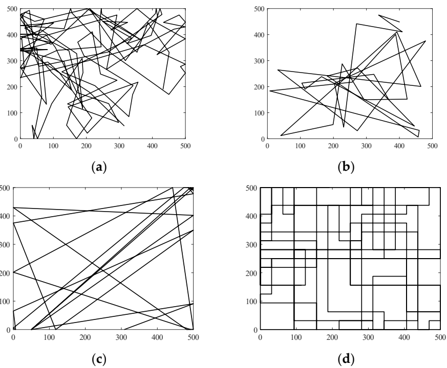
Figure 3. Pure randomized mobility trajectories: (a) Random Walk mobility model where each node selects a random direction [0, 2\pi) and speed S [ S_{min} , S_{max} ] that is maintained for a predefined time interval t or a constant distance d ( 500 \times 500 m, t = 5 s); (b) Random Waypoint ( T_{pause} = 3 s); (c) Random Direction, as in RWP but the node searches the edge point of the simulation area; and (d) Manhattan Grid with example of an urban scenario with 16 horizontal and 16 vertical streets.
