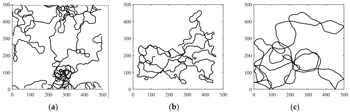
Figure 5. Time-Dependent mobility trajectories: (a) Boundless Simulation Area, (b) Gauss-Markov, and (c) Smooth Turn.
