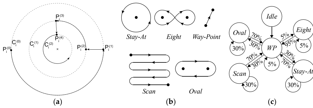
Figure 2. Path-Planned mobility trajectories: (a) Semi-Random circular mobility model; (b) Paparazzi autopilot UAV Movements ( Stay-At , Eight , Way-Point , Scan , and Oval ); and (c) PPRZM state machine.
