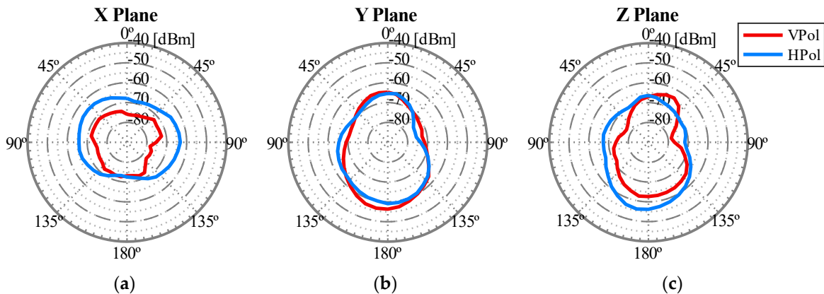
Figure 17. Radiation pattern of the WiTi on-board the UAV for the antennas configuration shown in Figure 13 in the U2G link working in 2.4 GHz: (a) X Plane, (b) Y Plane, and (c) Z Plane.
