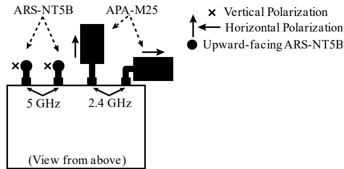
Figure 13. The best antenna configurations of the WiTi as seen from above: 2.4 GHz band for the U2G link with APA-M25 antennas in horizontal position with 90° between them and 5 GHz band for the U2U link with ARS-NT5B antennas in vertical position.
