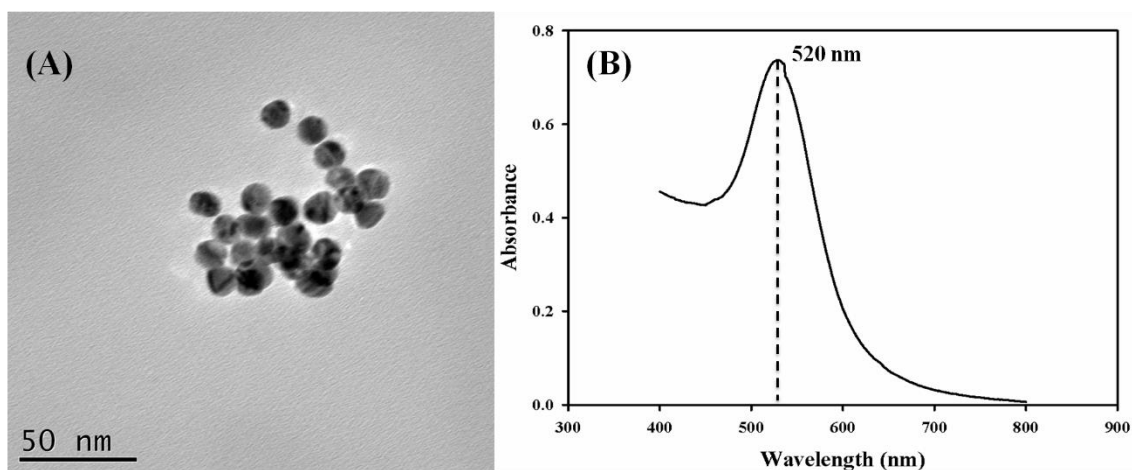
Figure S1. (A) TEM image of Au NPs. (B) UV-vis absorption spectrum of Au NPs in 1% of sodium citrate solution.
