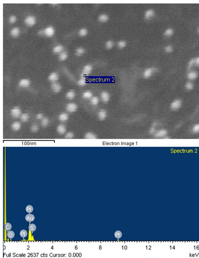
Figure S2. SEM/EDS analysis of the AuNPs-PEDOT/Pt electrode.
