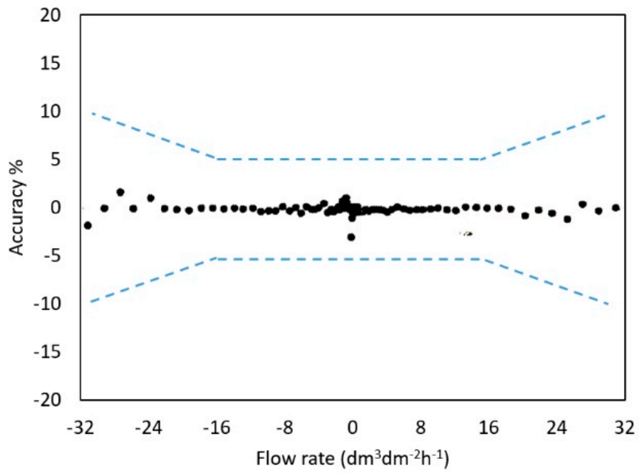
Figure S1. The accuracy expressed in percent is reported with the flow rate unit ( \text{dm}^3 \text{dm}^{-2} \text{h}^{-1} ) for the sap flow meter Sensirion, mod. SLQ-QT500. The accuracy test on the sensor is provided by the producer of the sensor, while the figure and the scale were adapted to our case study. .
