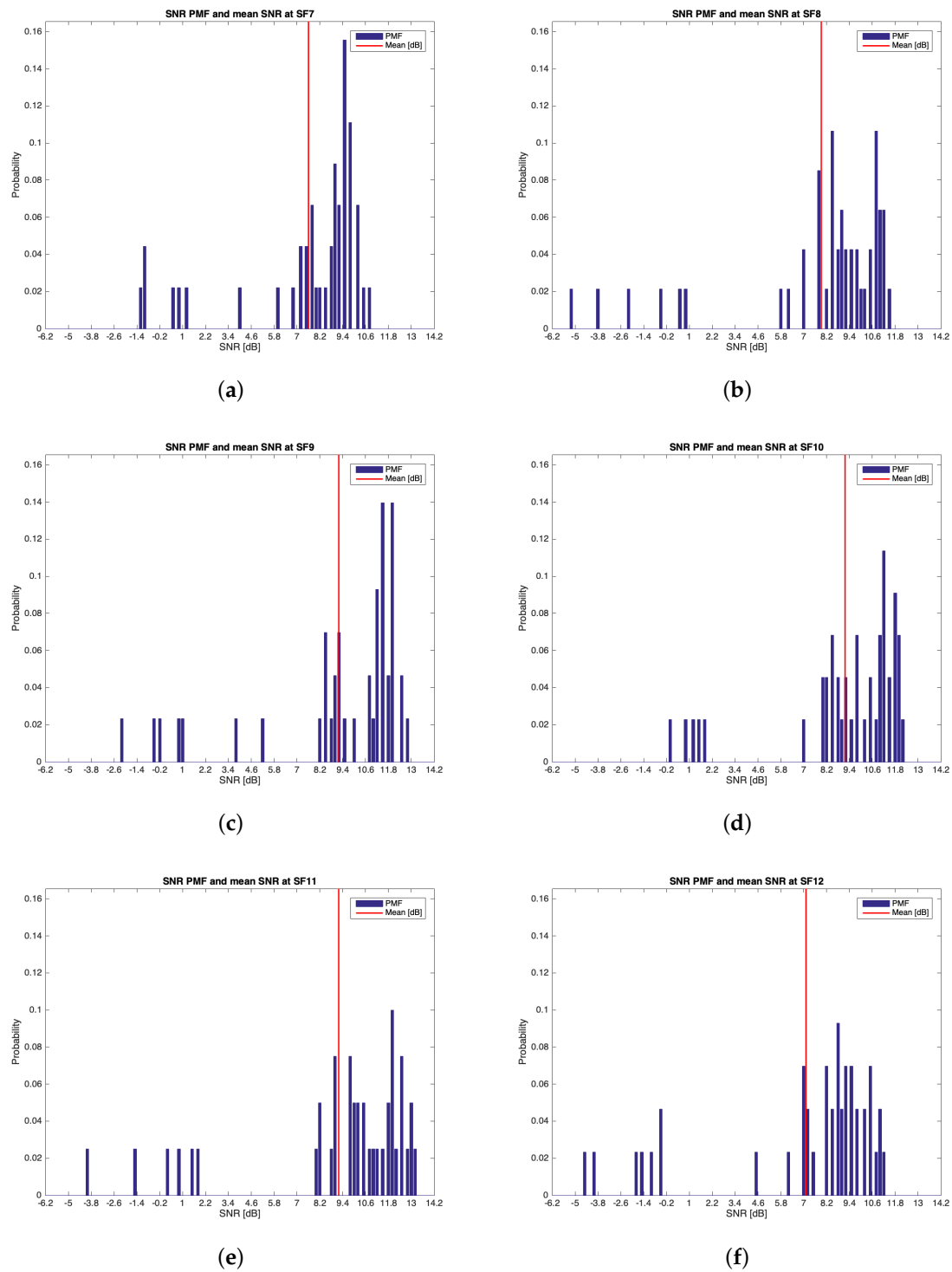
Figure 12. Group #1 SNRs PMFs: (a) SF = 7 ; (b) SF = 8 ; (c) SF = 9 ; (d) SF = 10 ; (e) SF = 11 ; (f) SF = 12 .
