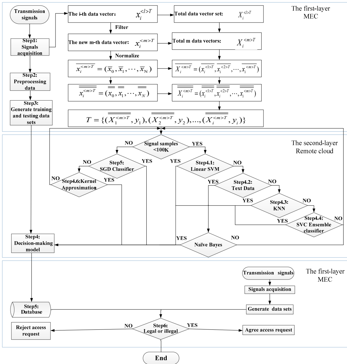
Figure 4. Flow chart of RFFID-MEC method algorithm.
