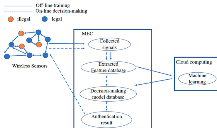
Figure 3. Detailed authentication process.
