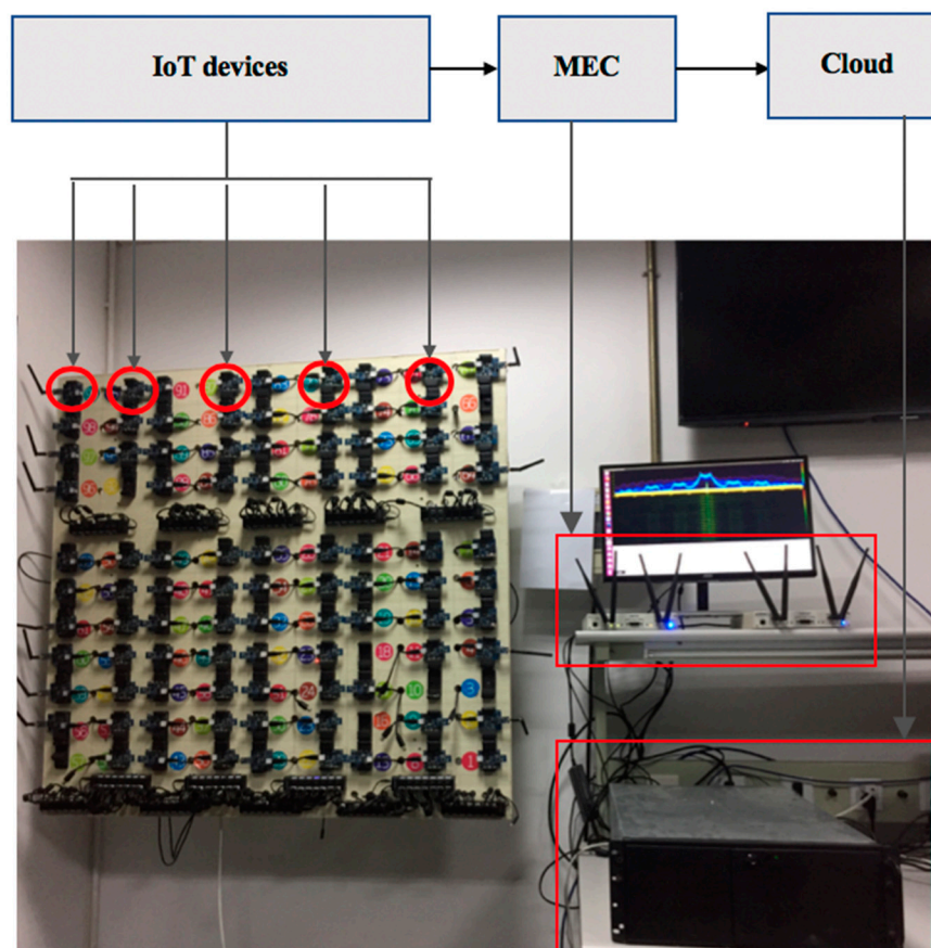
Figure 5. Typical application scenarios of RFFID-MEC authentication method.
