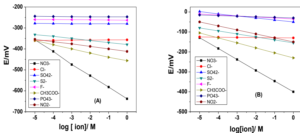
Figure S1. The plots and Nernstian slopes for the measured ions using (A) GC/MWCNTs/NO 3 - -ISE; and (B) GC/NO 3 - -ISE.
