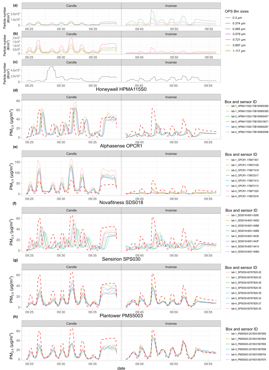
Figure A10. Time series of experiment 2. From top to bottom: (a,b) TSI 3330 OPS Bin size distribution; (c) Nanotracer ultrafine particles number concentration \#/\text{cm}^3 ; (d–h) \text{PM}_{2.5} of the sensors for each model of sensor, against DustTrak (red dotted line). The sensors are named according to the box they are placed in and their serial number.
