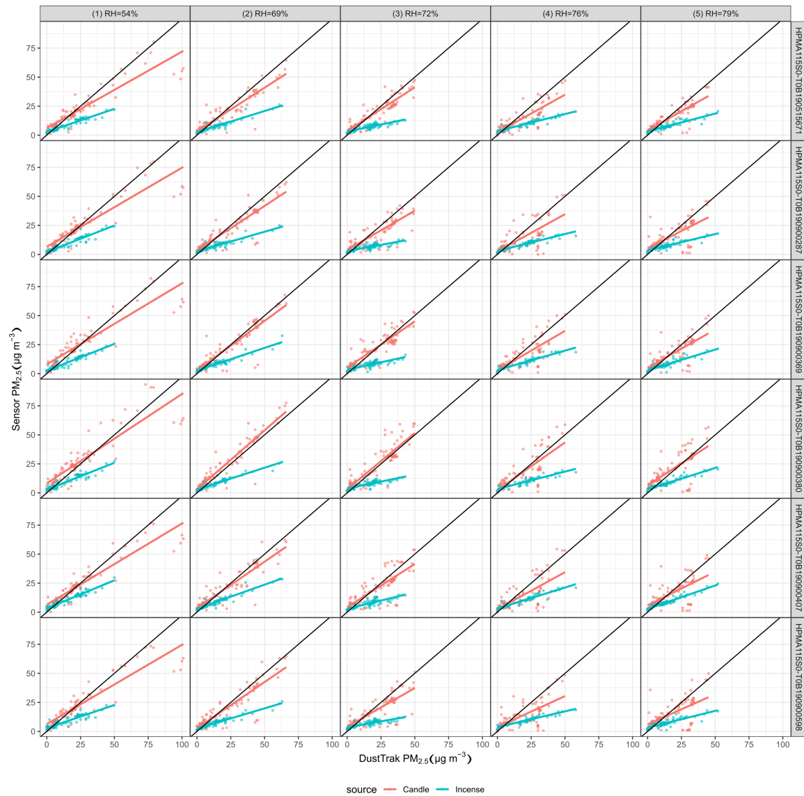
Figure A9. Comparison and linear regression of the Honeywell HPM115S0 with the DustTrak ( x = \text{DustTrak} , y = \text{sensors} ) during the five experiments for peaks and stable concentrations of PM generated using incense and candle. The black line is x = y .
