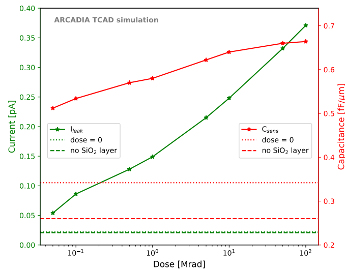
Figure 12. Leakage current I_{leak} (green) and sensor capacitance C_{sens} (red) as a function of the total ionizing dose for a 50 \mu\text{m} thick microstrip sensor. The values obtained in simulations with and without the \text{SiO}_2 layer in the absence of irradiation are shown as horizontal lines and referred to as “dose = 0” and “no \text{SiO}_2 layer”, respectively.
