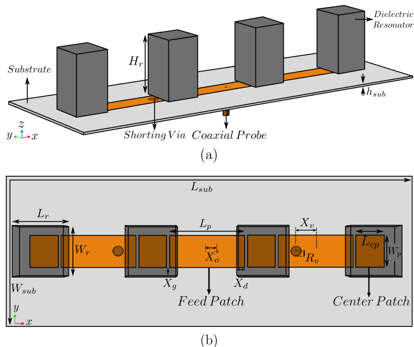
Figure 6. Schematic diagram of proposed four-element standing-wave DRA array: (a) 3D view and (b) top view with transparent resonators.
