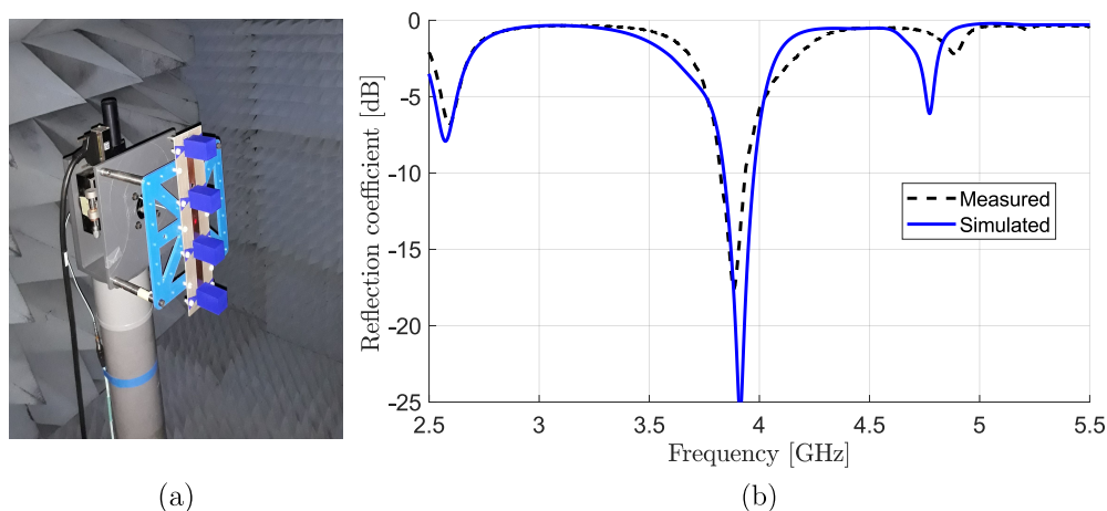
Figure 11. (a) Manufactured prototype of four-element DRA array. (b) Measured and simulated S_{11} of manufactured four-element standing-wave DRA array prototype.
