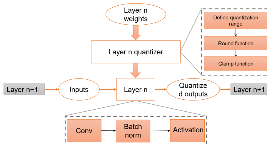
Figure 4. Overview of the proposed methodology. Each layer’s weight is passed through the quantizer. After defining the quantization range, the parameters are passed through two functions (round and clamp).
