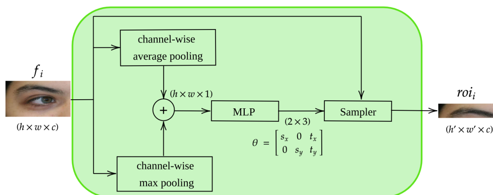
Figure 3. Detailed architecture of the Spatial transformation module. The input convolutional feature map f_i first undergoes two channel-wise pooling operations (maximum and average) to highlight the most discriminative spatial areas. Their outputs are then added together and passed to a multi-layer perceptron to learn \theta - the transformation matrix. \theta is used to sample a region of interest from f_i , which will be processed by the local branches. Although the Spatial transformation module operates on intermediate feature maps, for illustration purposes we exemplify its function with an image (corresponding to the input feature map).
