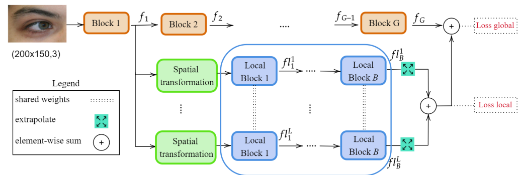
Figure 2. The overview of the proposed deep learning model based on convolutional neural networks. The input image is processed using several global and local convolutional blocks. Block and Local Block refer to the convolutional blocks/layers in the global branch (depicted in orange) and local branch (depicted in blue), respectively. The feature map f_i from some level i in the network architecture is fed to L \geq 1 local branches. Each branch applies a Spatial transformation module to select an ROI within the input feature map, and then further analyses this region by applying several shared convolutional blocks. In the end, the feature maps of the local branches are extrapolated to the same size and fused with the global branch via element-wise summation. To ensure that the local branches extract useful features, the loss function is applied to both the global branch and the summation of the local branches.
