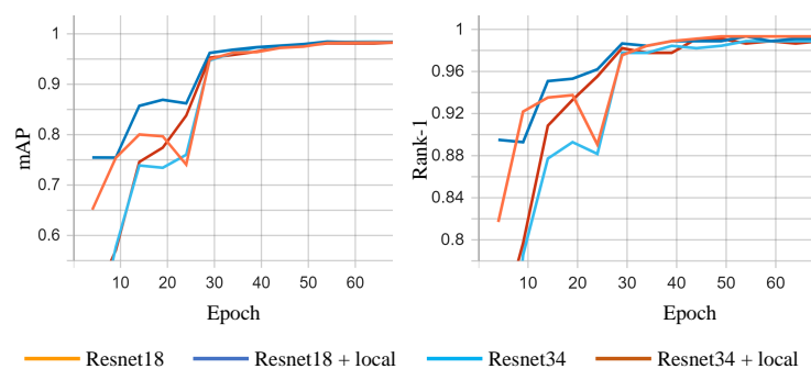
Figure 5. Metrics mAP (mean Average Precision) and rank-1 evolution during the training process for the closed-world setting.
